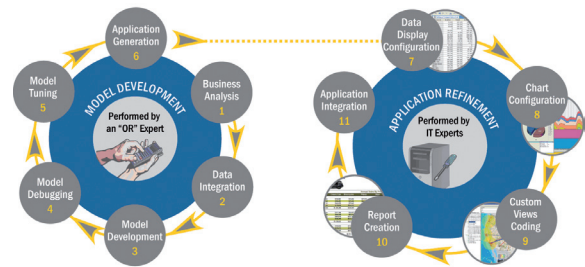
Figure 5: The Complete Custom Planning and Scheduling Application Development Process
