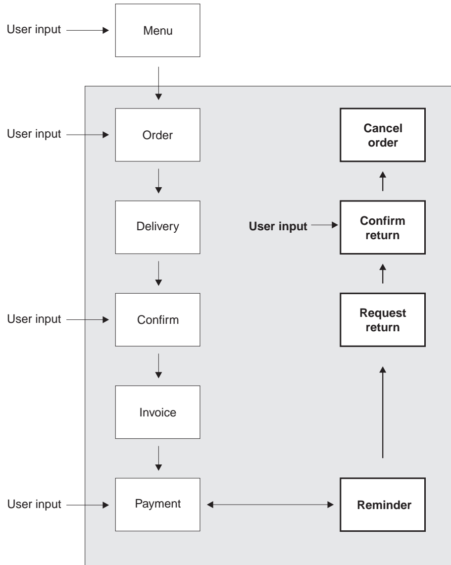
Figure 26. Process flow with compensation actions included. (The root activity is not shown.) Changes from the user-related example described in Chapter 7 are shown in bold.
