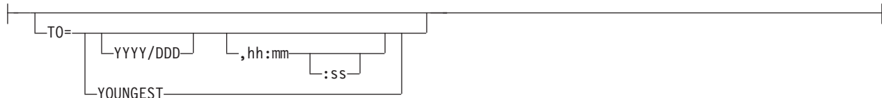
Figure 8. Log stream SUBSYS data set specification
