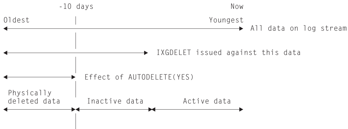
Figure 9. Active and inactive data on a log stream. The log stream has been defined with a RETPD value of 10.
