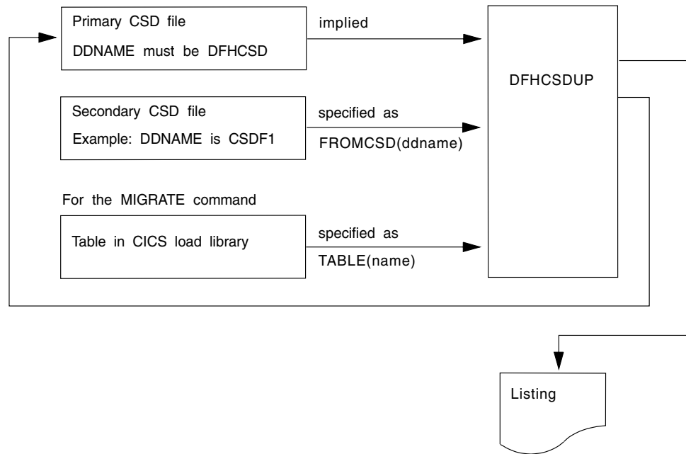
Figure 28. The DFHCSDUP offline utility program
