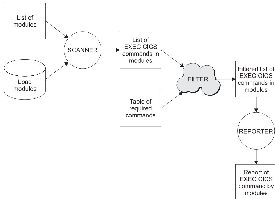
Figure 31. Load module scanner with filter
