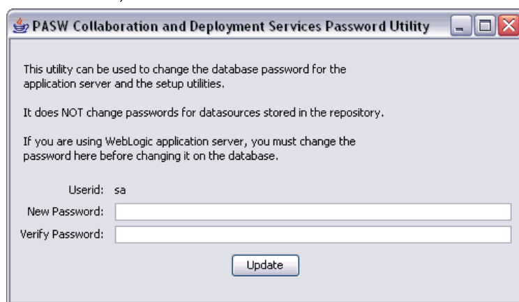
Figure 3-10 Password Utility
