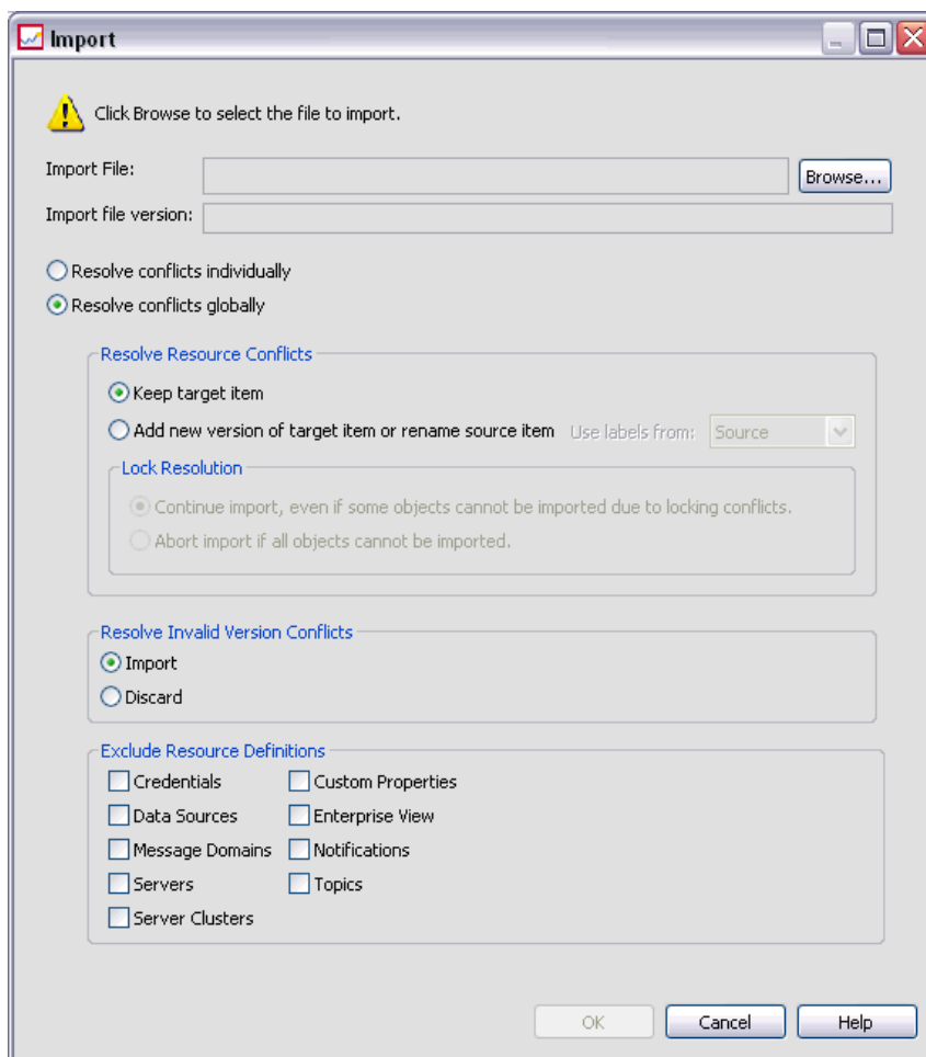
Figure 4-18 Resolving import conflicts globally or individually
