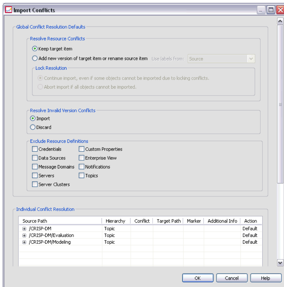
Figure 4-21 Resolving import conflicts
