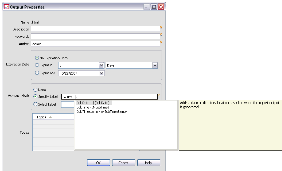
Figure 3-2 Output Properties dialog when selecting a JobDate variable using content assist
