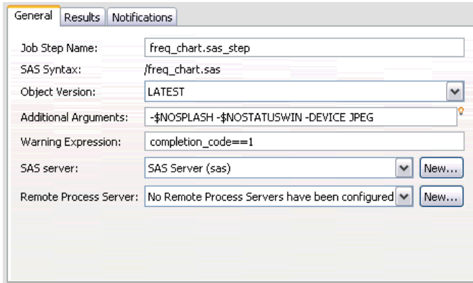
Figure 15-8 General tab with DEVICE option
