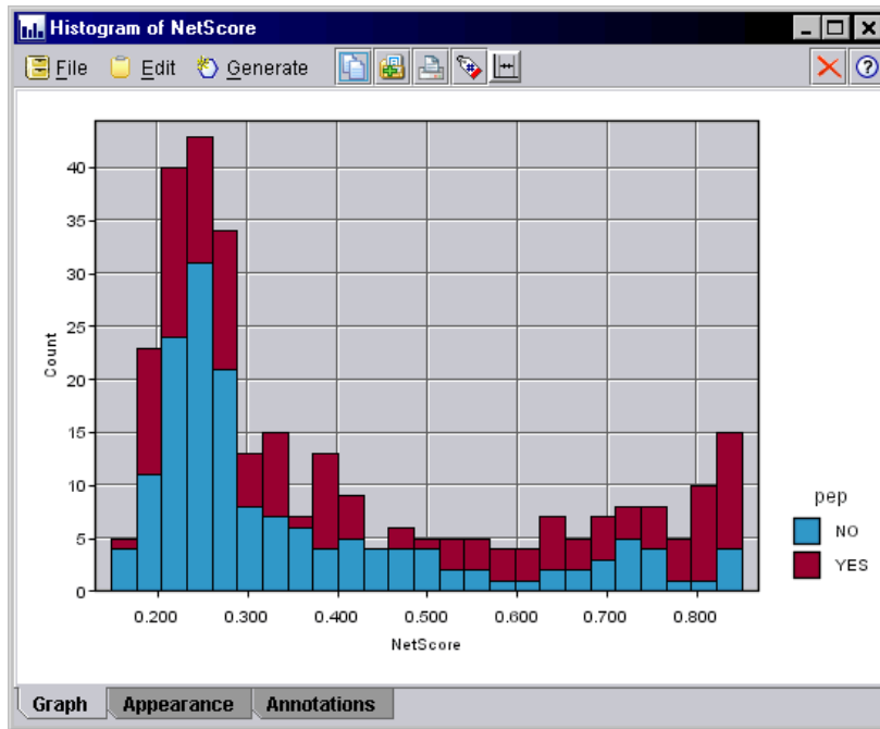
Figure 13-7 Sample histogram
