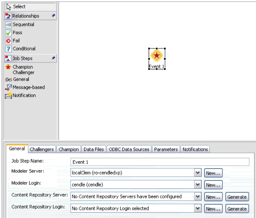
Figure 18-1 Champion challenger work on the job canvas
