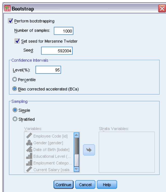
Figure 3-9 Bootstrap dialog
