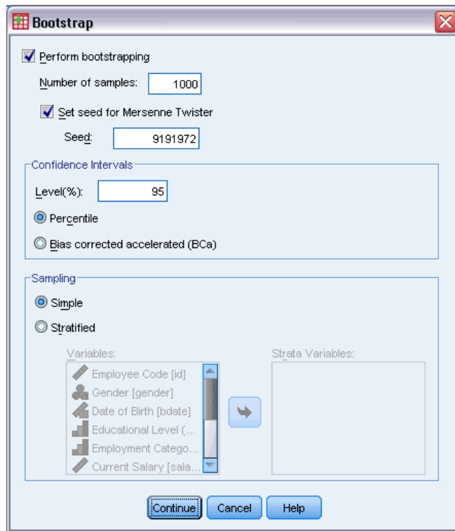
Figure 3-17 Bootstrap dialog
