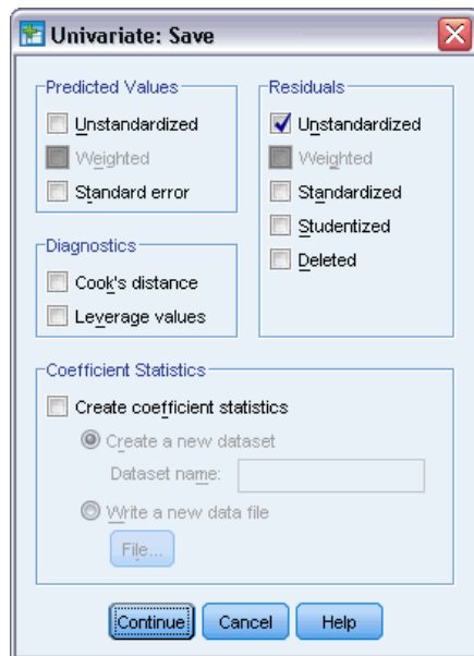
Figure 3-14 Save dialog
