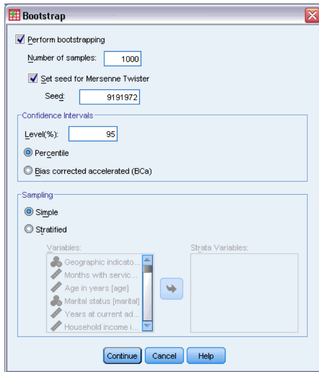
Figure 3-4 Bootstrap dialog
