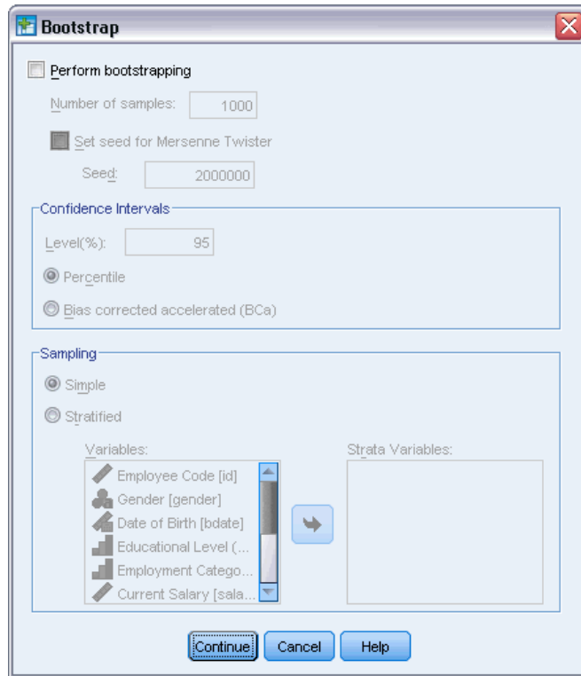
Figure 3-15 Bootstrap dialog
