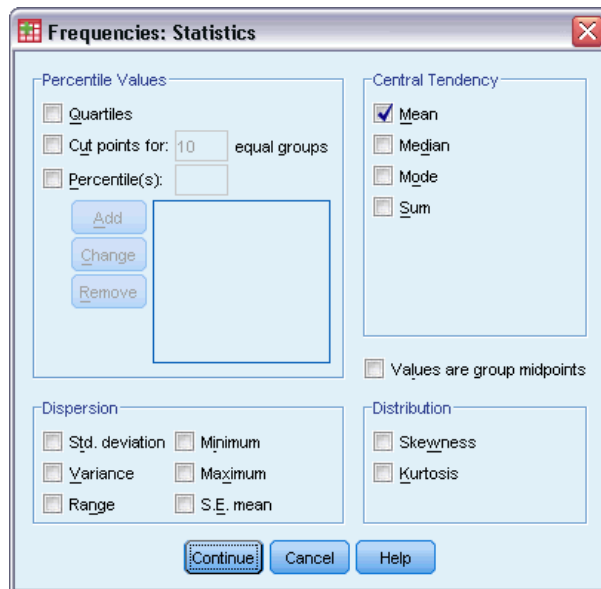
Figure 3-3 Statistics dialog
