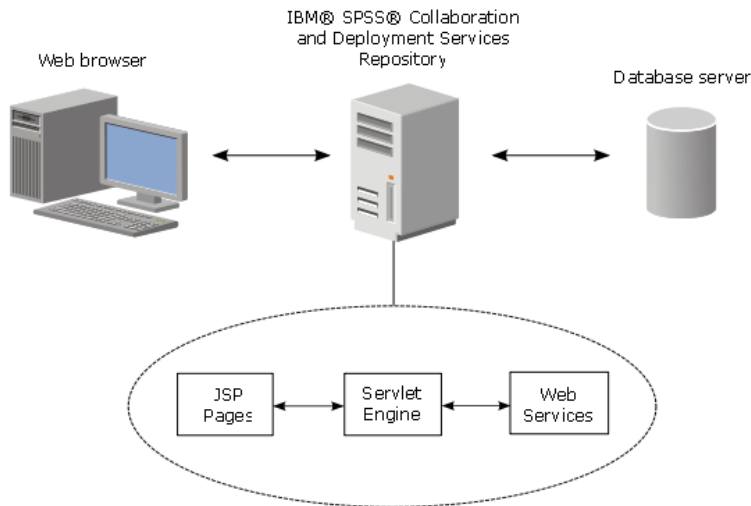
Figure 1. Architecture JSP
