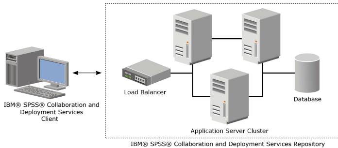
Figure 5. Cluster architecture
