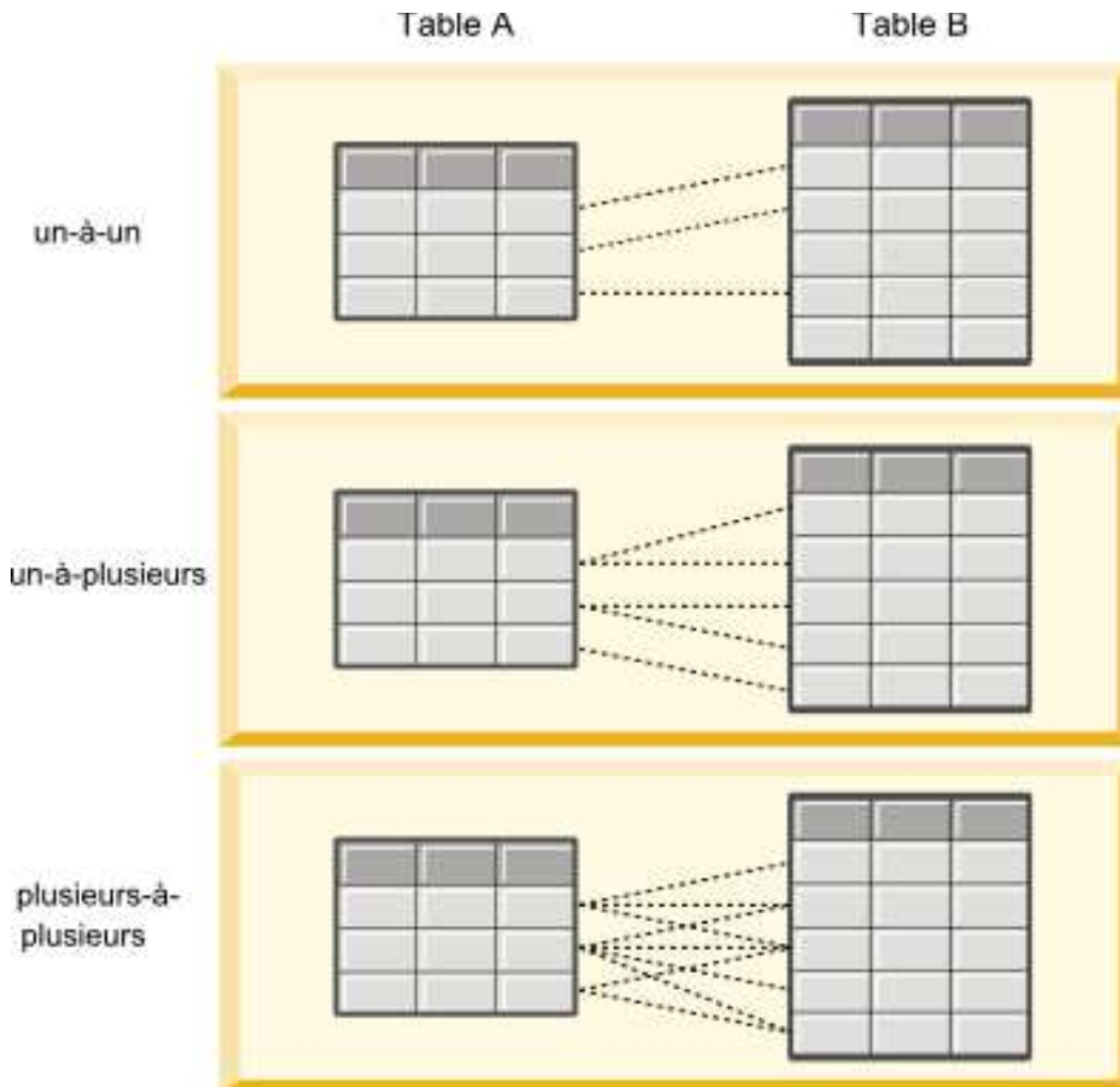
Figure 4. Types des relations de tables
