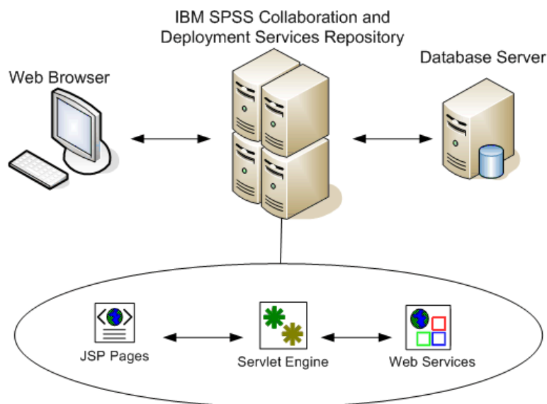
Figure 4-1 JSP Architecture
