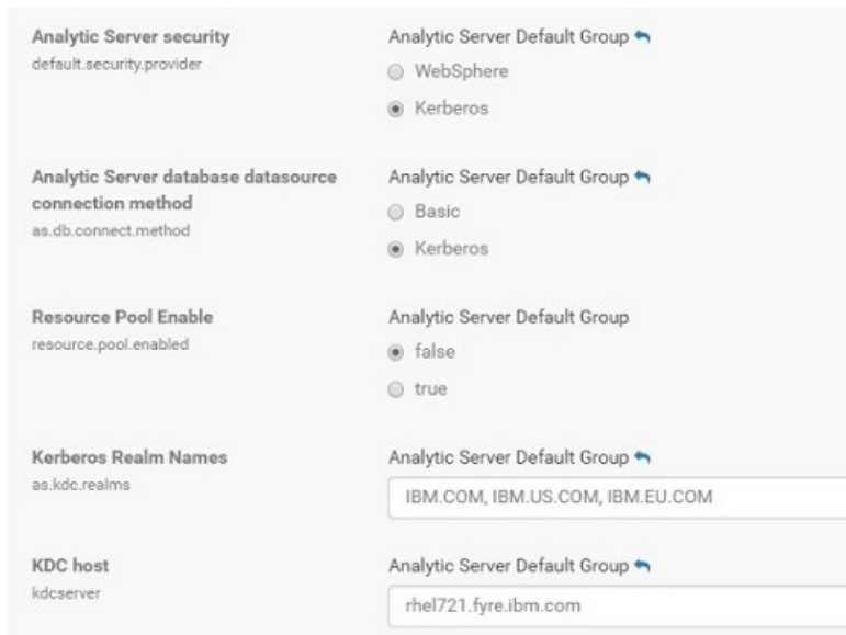
Figure 7: Example Kerberos settings
