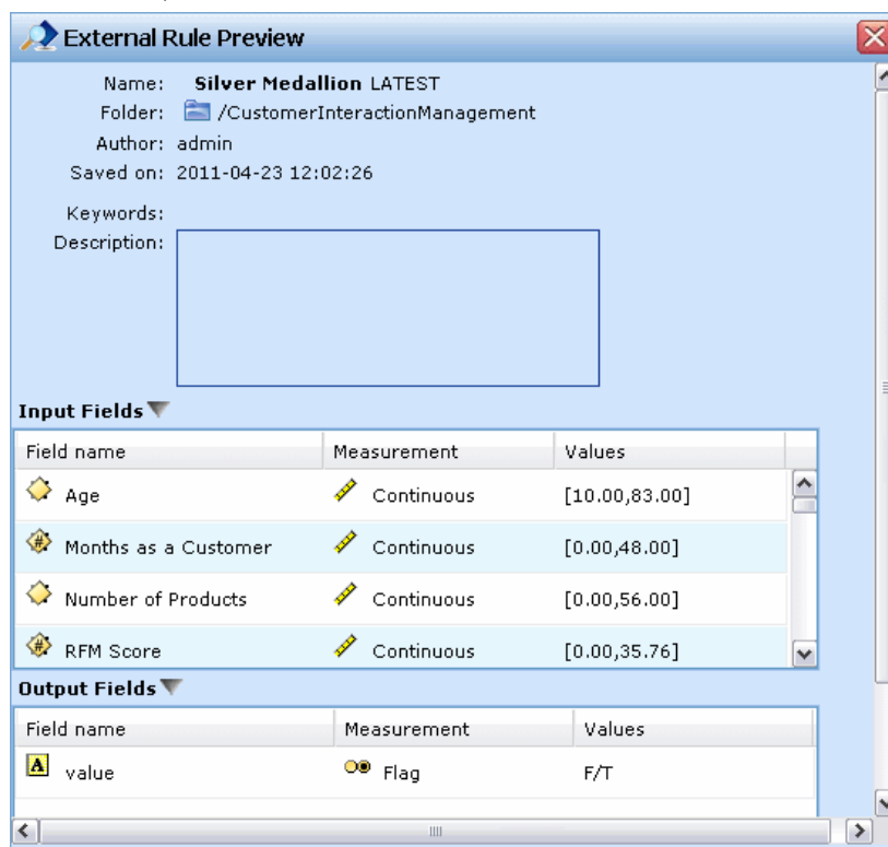
Figure 4-15 External rule preview
