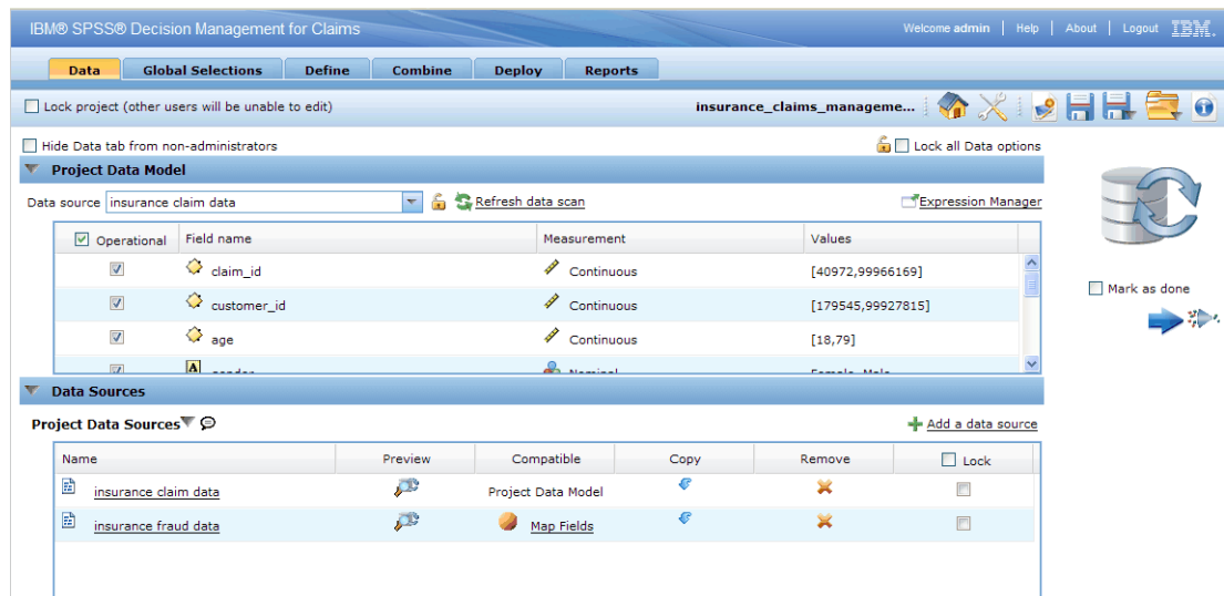
Figure 6-3 Administrator options on the Data tab
