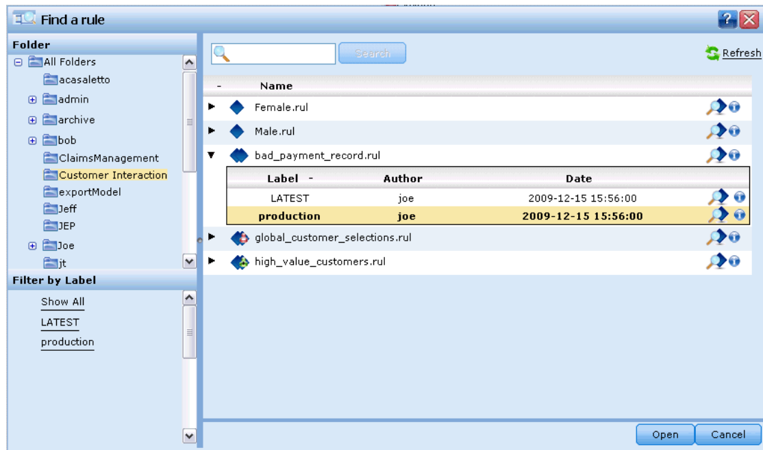
Figure 2-15 Finding an existing rule
