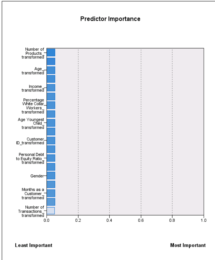
Figure 5-5 Variable Importance chart
