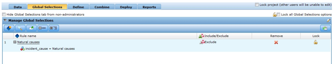
Figure 4. Global selections
