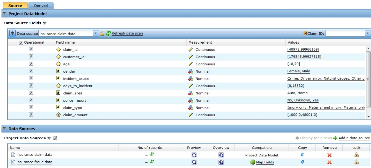
Figure 3. Data tab
