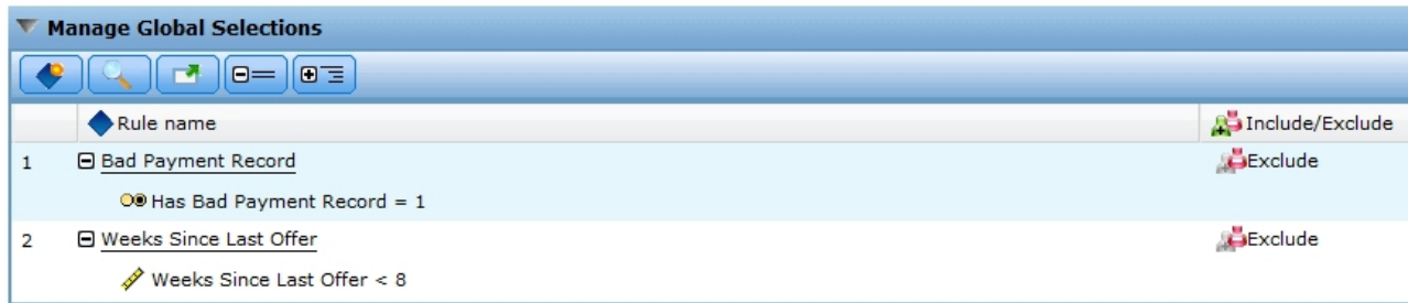
Figure 4. Global selections
