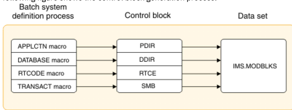
Figure 4. Control block generation process for MODBLKS resources
