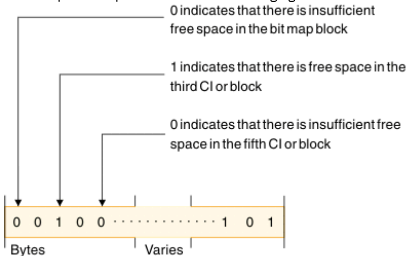
Figure 46. Bitmap for HD databases
