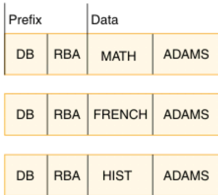
Figure 179. Examples of source segments for each student
