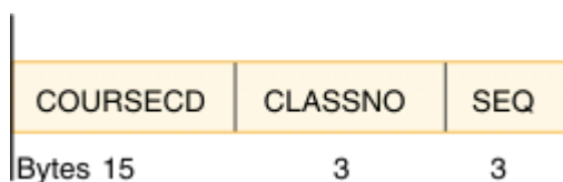
Figure 187. Concatenated key of the STUDENT segment
