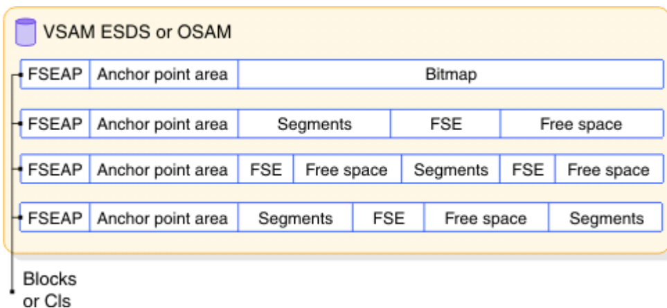
Figure 45. Format of an HD database and special fields in it
