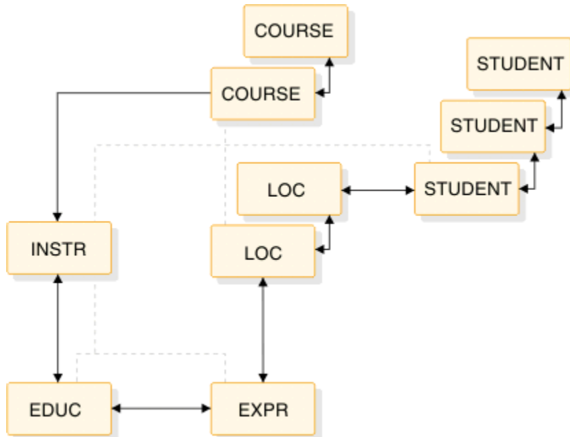
Figure 38. Hierarchical forward and backward pointers
