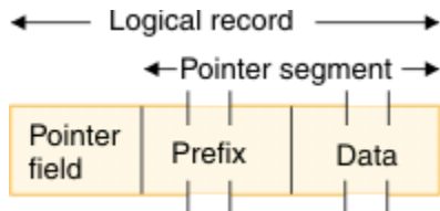
Figure 180. Example of a logical record containing a pointer segment
