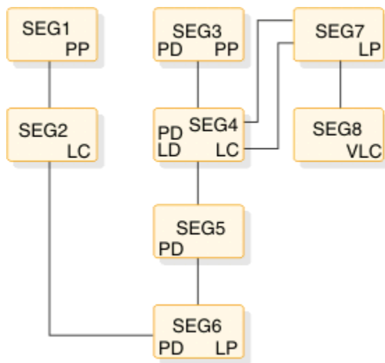
Figure 165. Third access path example
