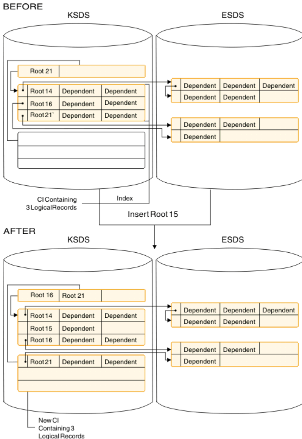
Figure 28. Inserting a root segment into a HISAM database (no free logical record exists in the CI)
