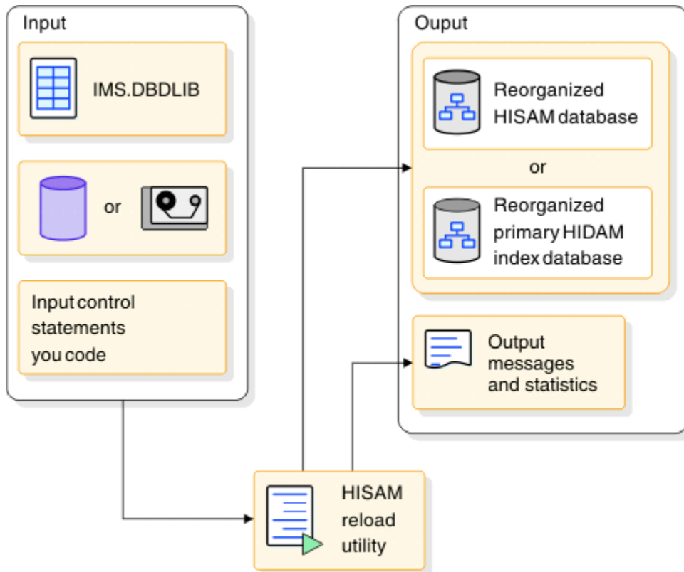
Figure 251. HISAM Reorganization Reload utility (DFSURRLO)
