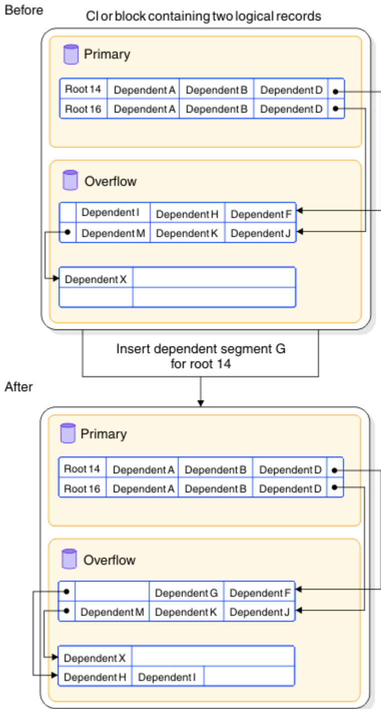
Figure 30. Inserting a dependent segment into a HISAM database (no space exists in the logical record)
