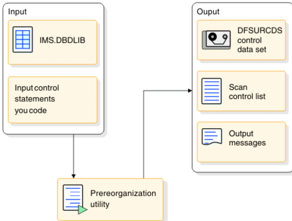
Figure 254. Database Prereorganization utility (DFSURPRO)
