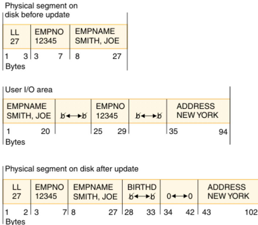
Figure 205. Second example of a missing field on a replace call
