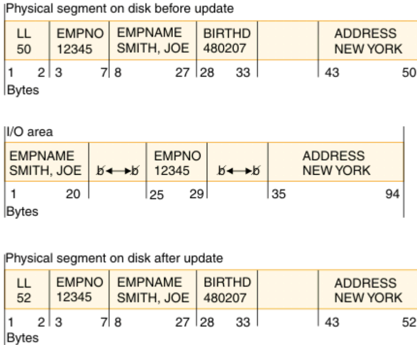
Figure 208. Example of a partially present field on a REPL call
