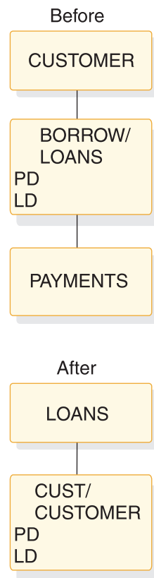
Figure 149. Logical child, virtual pairing—virtual delete rule example: before and after
