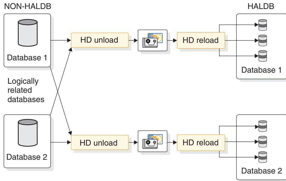
Figure 316. Migrating databases with logical relationships
