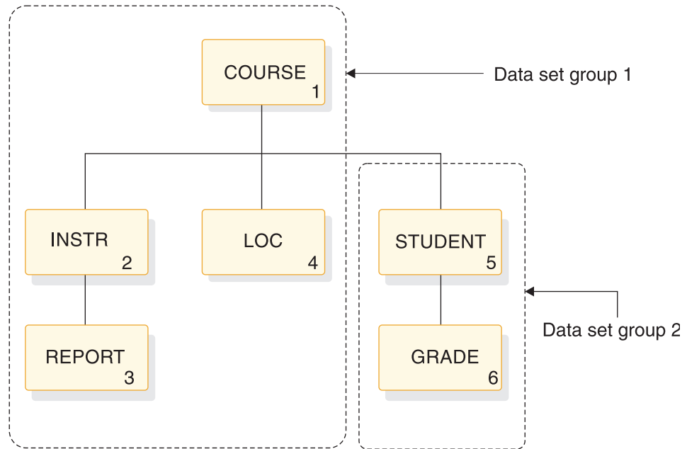
Figure 209. Database record split into two database groups
