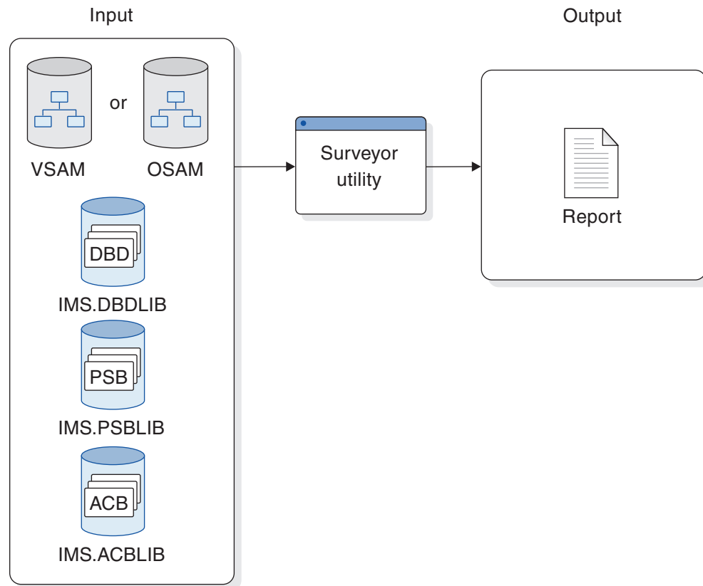
Figure 266. Database Surveyor utility (DFSPRSUR)
