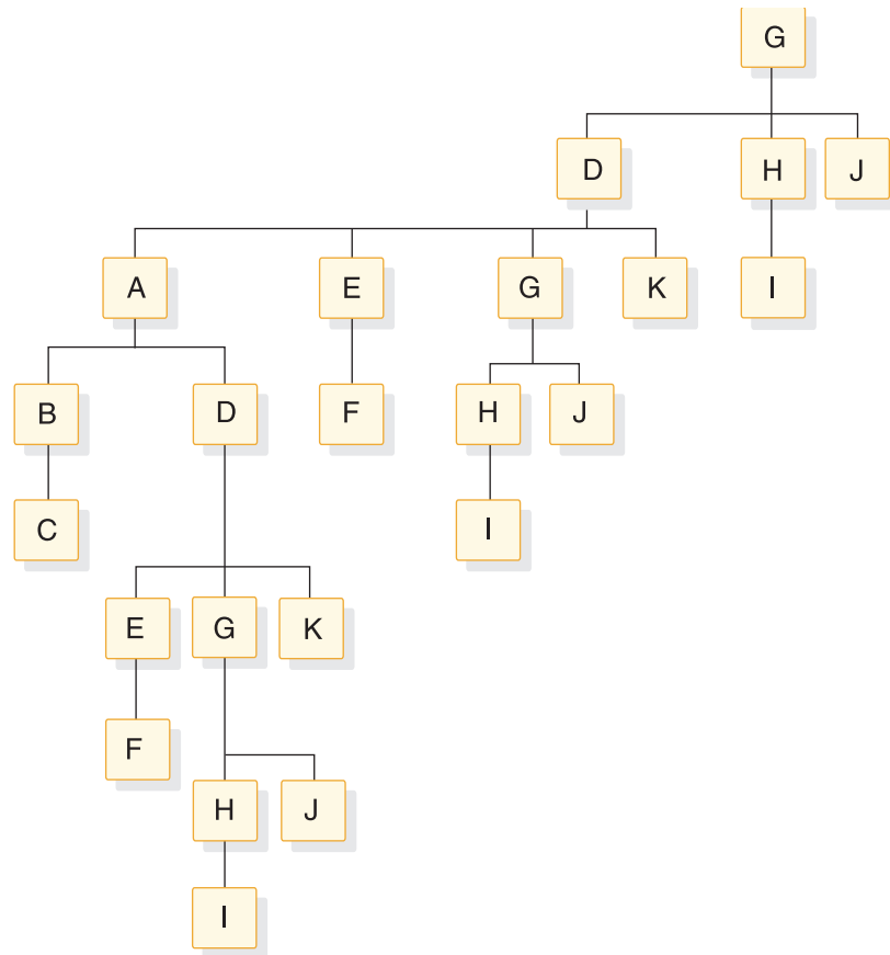
Figure 175. Secondary index structure indexed in secondary index on segment G
