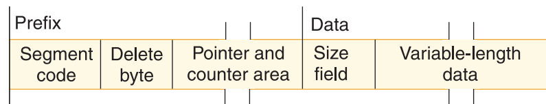
Figure 196. Format of HISAM variable-length segments
