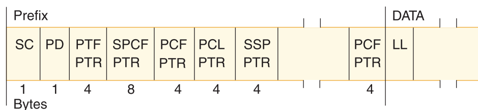
Figure 60. Root segment format (with sequential and direct dependent segments with subset pointers)
