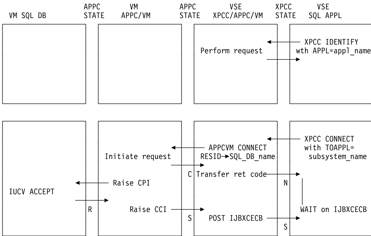
Figure 240. Successful XPCCV CONNECT
