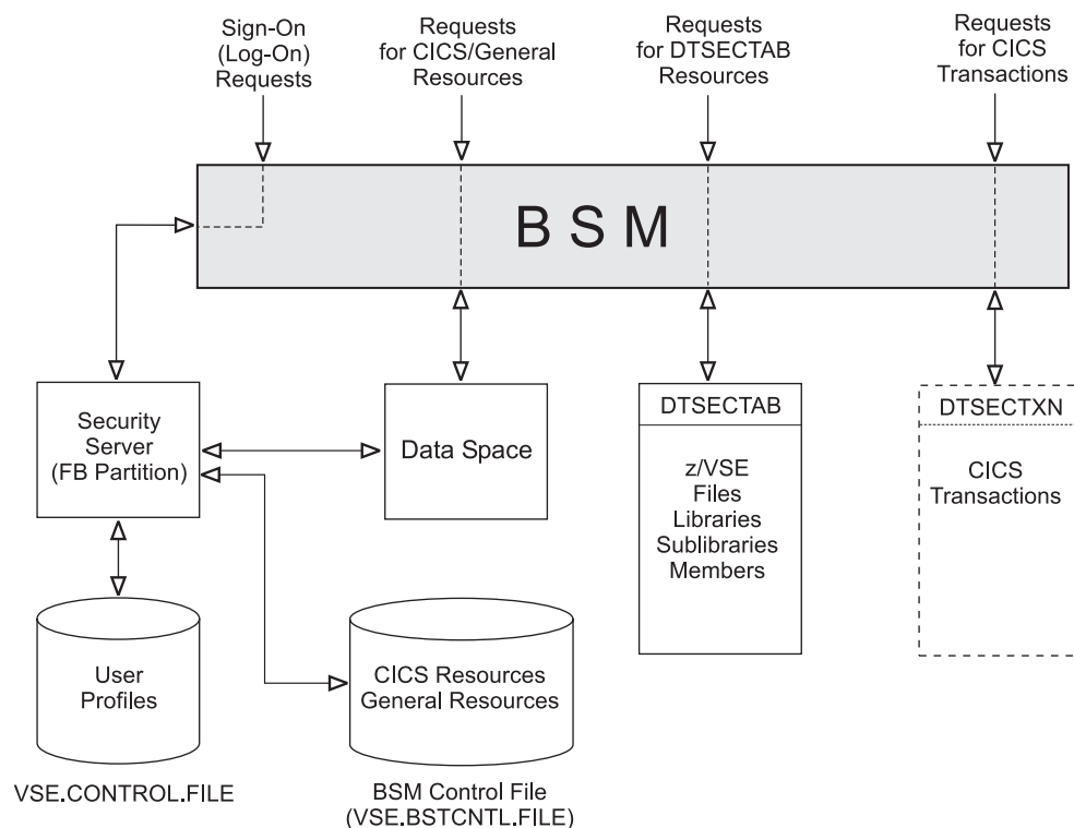
Figure 22. Logical Structure of BSM Security Support
