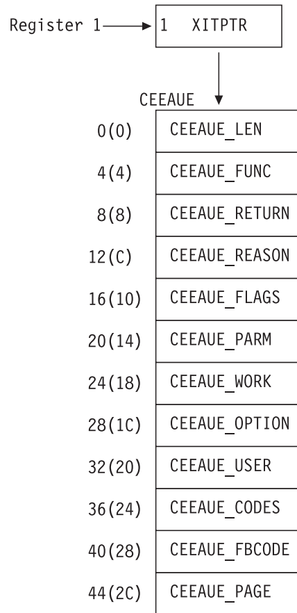
Figure 19. Interface for CEEBXITA Assembler User Exit
