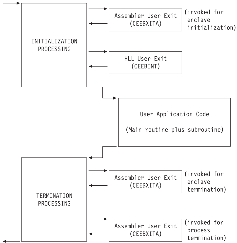
Figure 18. Location of User Exits
