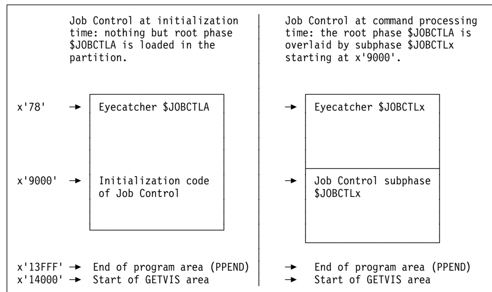
Figure 47. Job Control Storage Layout
