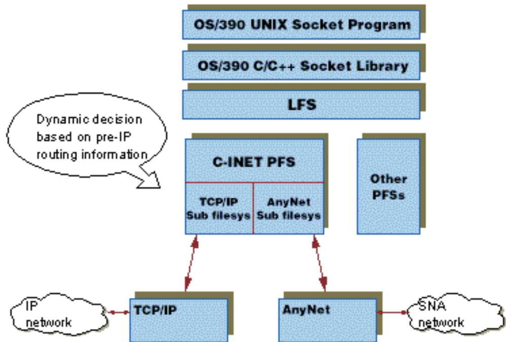
Figure 3. Common sockets
