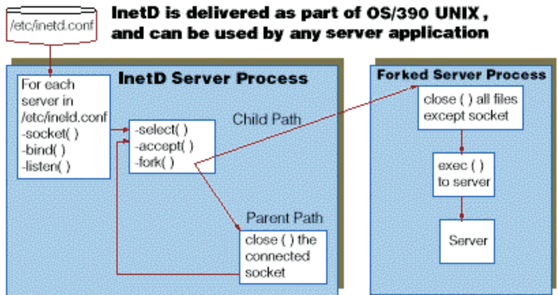
Figure 4. INETD Overview
