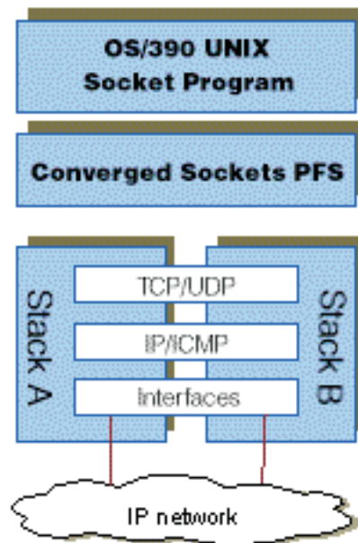
Figure 4. Converged Stacks As Perceived by OS/390 UNIX Applications
