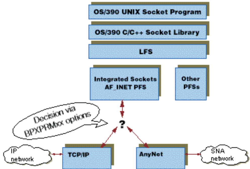
Figure 2. Integrated sockets
