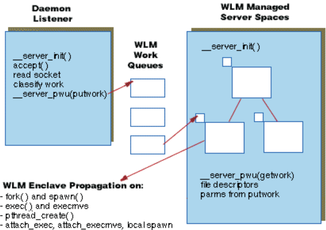
Figure 3. Using the WLM Server Services
