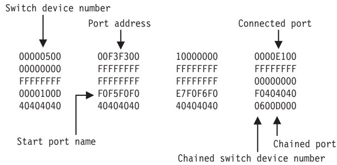
Figure 12. QUERY SWITCH Command - Sample Output.
