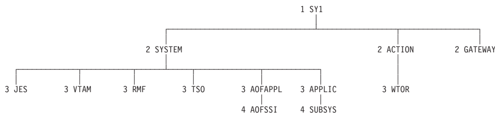
Figure 18. SDF Example: Hierarchy Defined by SY1 Tree Structure. The diagram shows how the order of dependence relates to level number.
