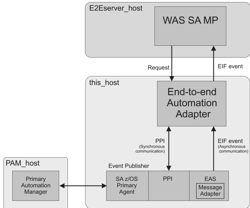
Figure 2. End-to-end automation adapter communication
