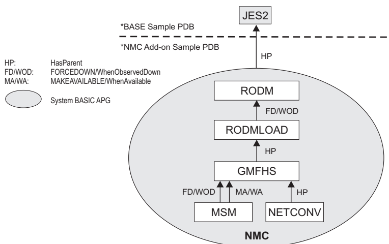
Figure 21. Environment for the SA z/OS Topology Manager
