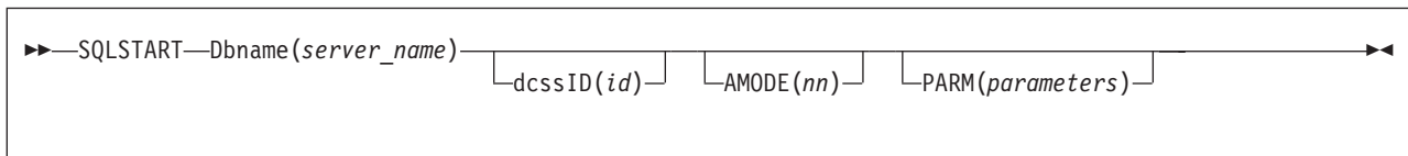
Figure 10. SQLSTART EXEC
