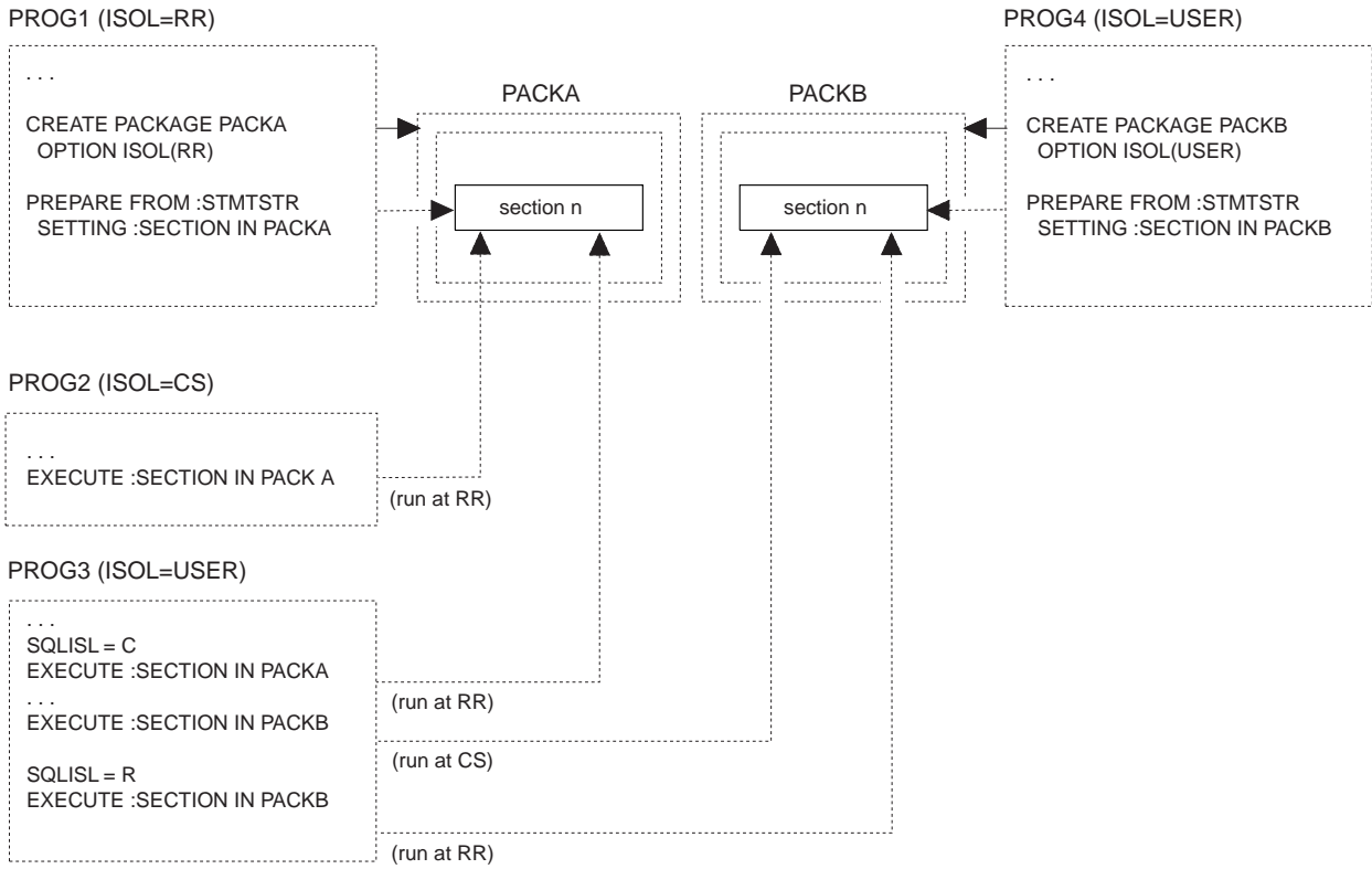
Figure 129. Version 3 Release 1
