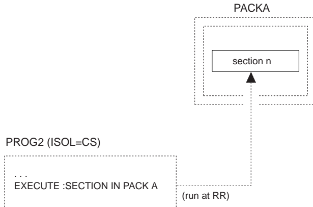
Figure 132. Re-preprocessing PROG2
