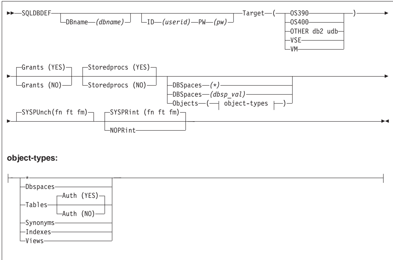
Figure 126. SQLDBDEF Utility
