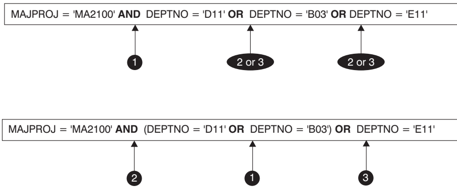
Figure 12. Search Conditions Evaluation Order
