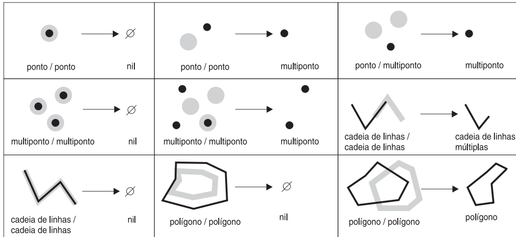
Figura 53. ST_Difference
