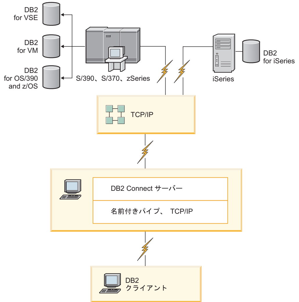
図 5. DB2 Connect Enterprise Edition
