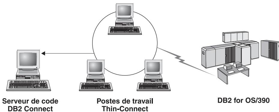
Figure 2. Topologie de client partiel standard utilisant DB2 Connect Personal Edition
