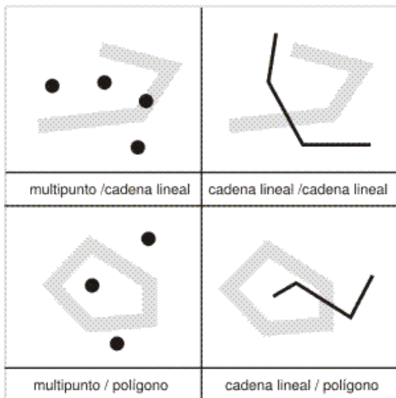
Figura 46. ST_Crosses
