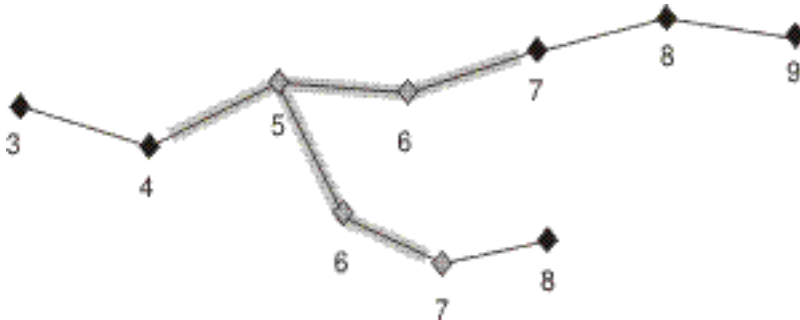
Figura 56. LocateBetween
