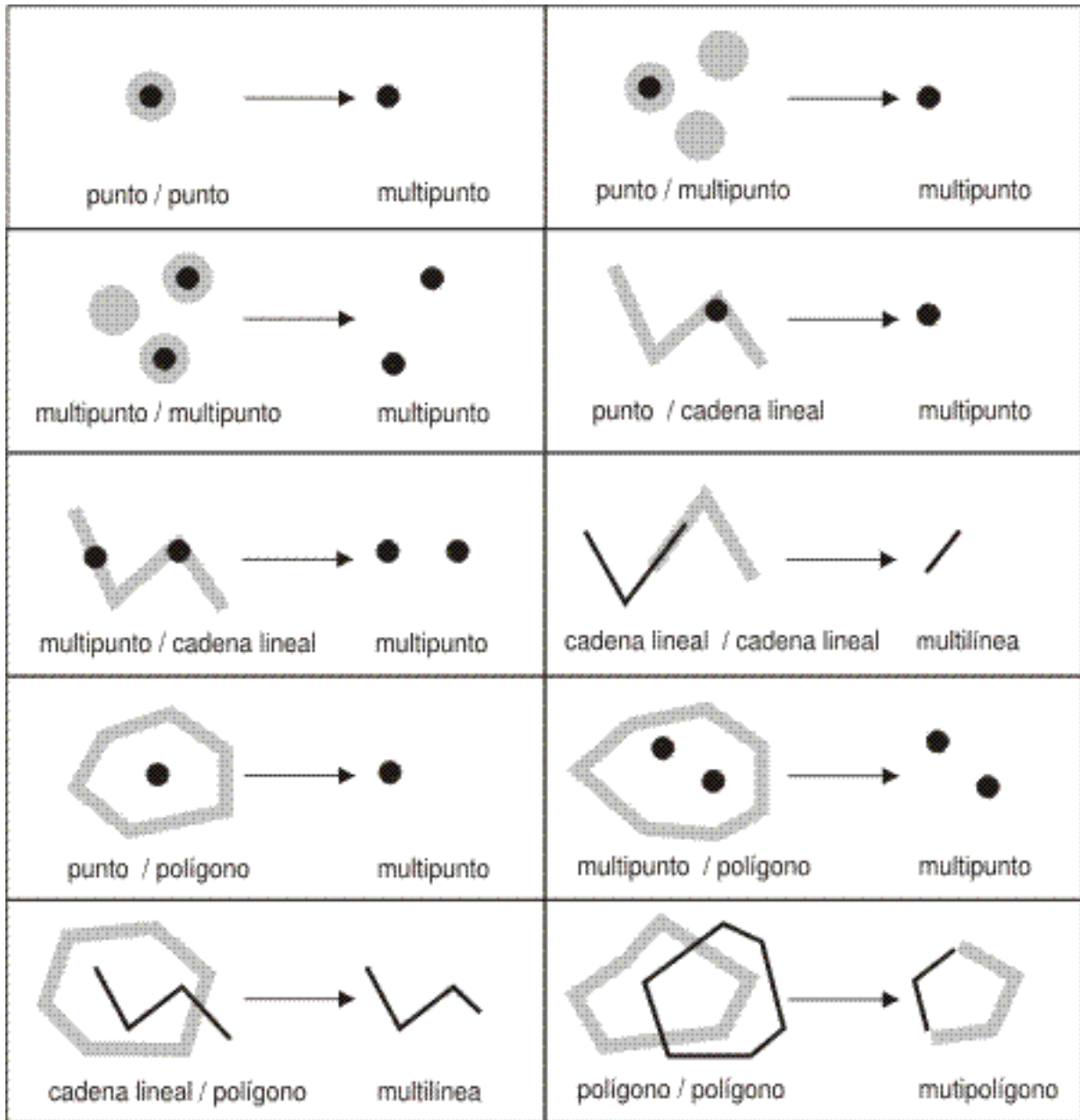
Figura 54. ST_Intersection
