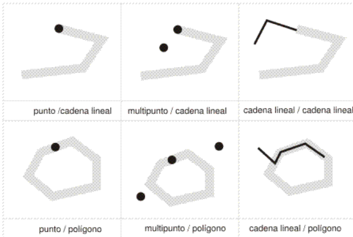
Figura 48. ST_Touches
