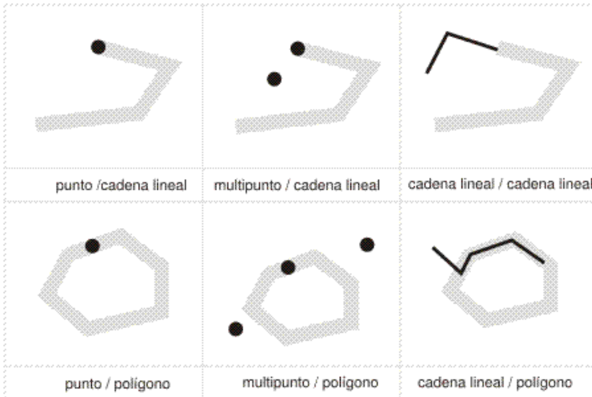
Figura 48. ST_Touches
