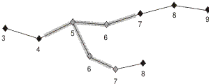
Figura 56. LocateBetween
