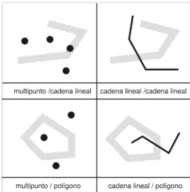
Figura 46. ST_Crosses
