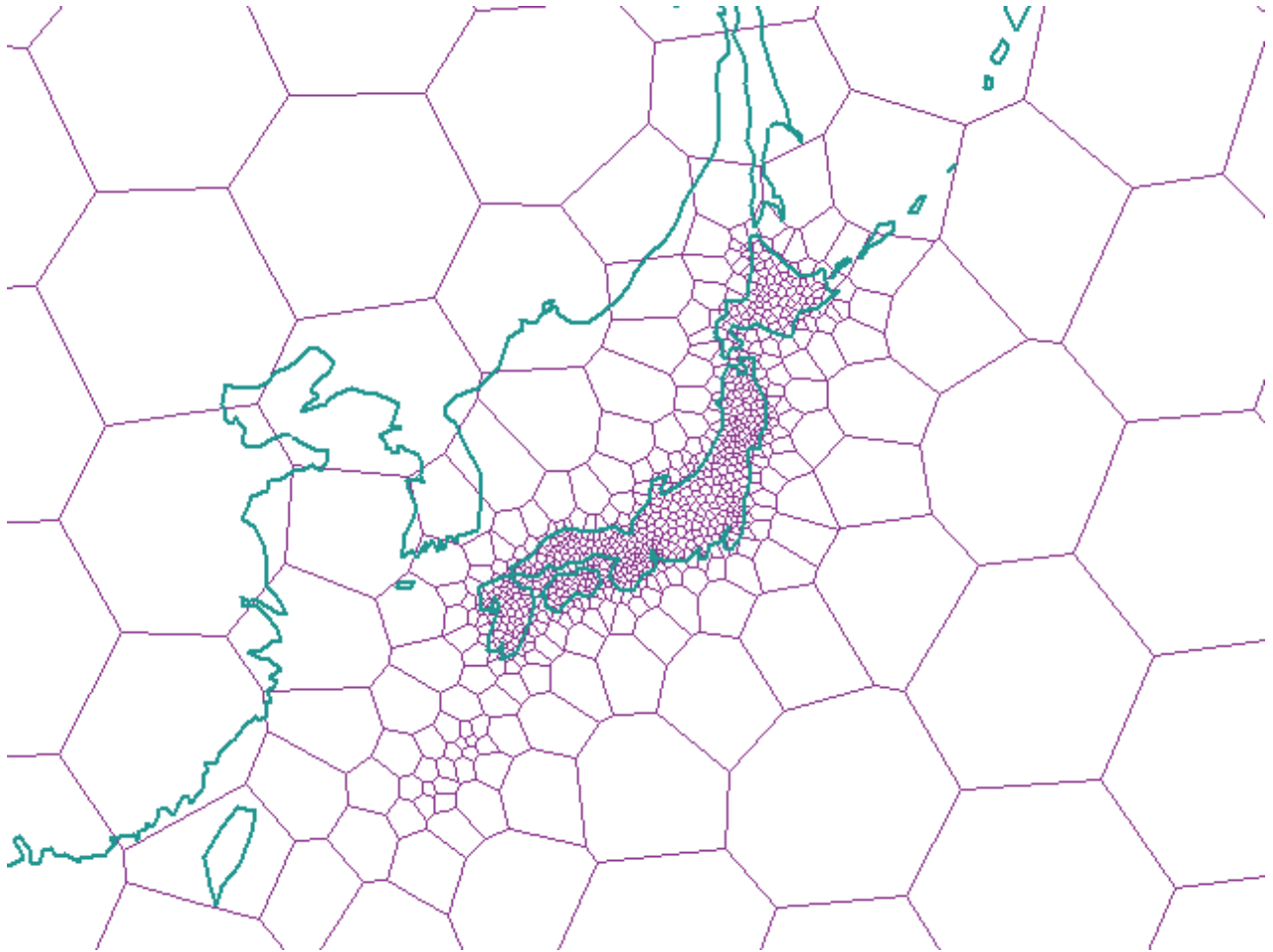
Figure 26. Voronoi cell structure for Japan
