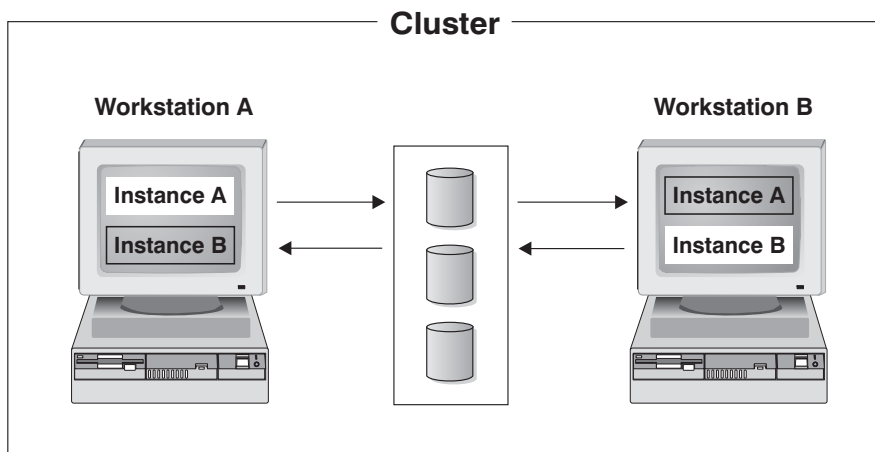
Figure 5. Mutual Takeover Configuration
