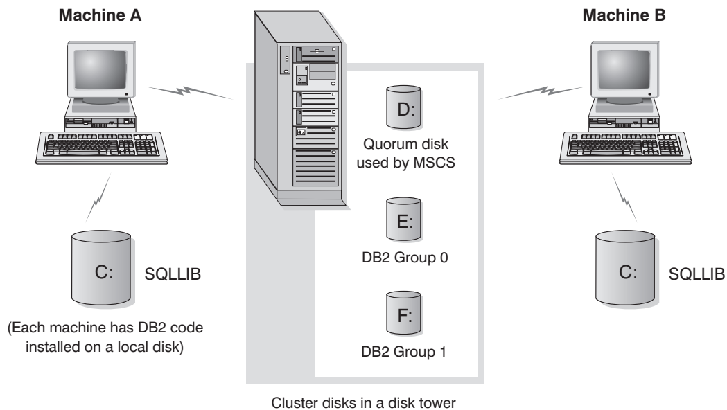
Figure 3. Example MSCS Configuration
