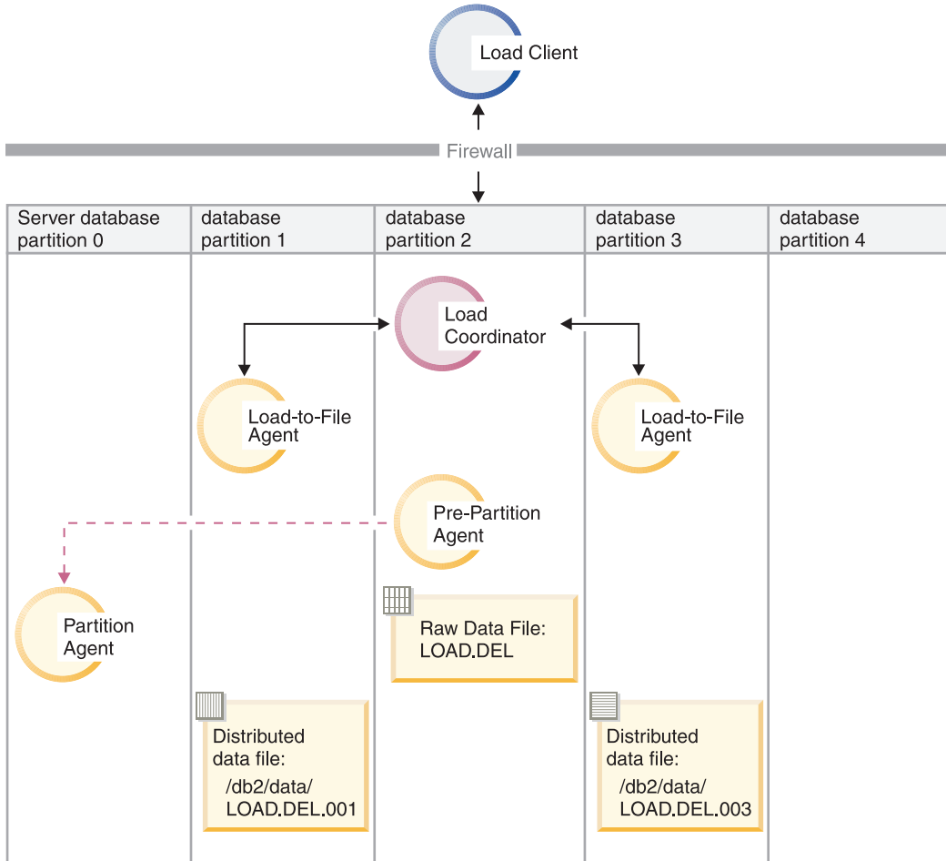
Figure 15. This diagram illustrates the behavior that results when the previous command is issued. Data is loaded into database partitions 1 and 3, using 1 partitioning agent running on database partition 0.
