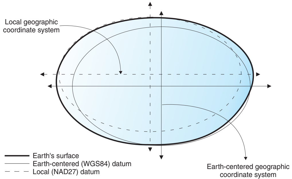
Figure 11. Datum alignments
