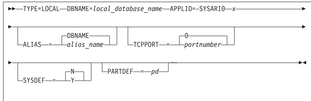
Figure 8. LOCAL Type Entry
