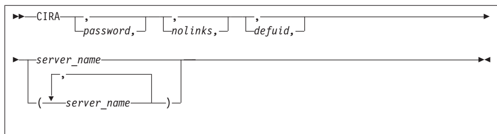
Figure 34. CIRA Transaction Syntax
