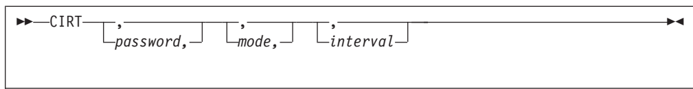
Figure 53. CIRT Transaction Syntax
