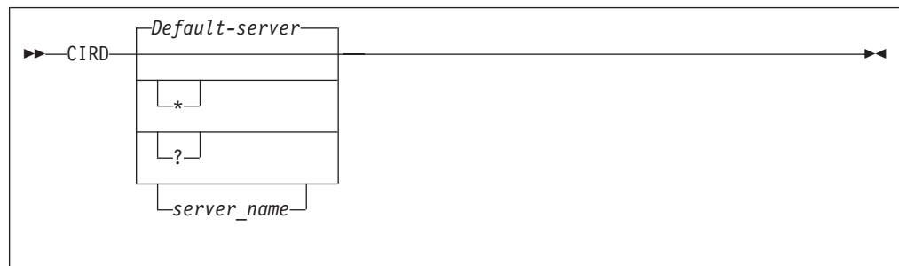
Figure 45. CIRD Transaction Syntax
