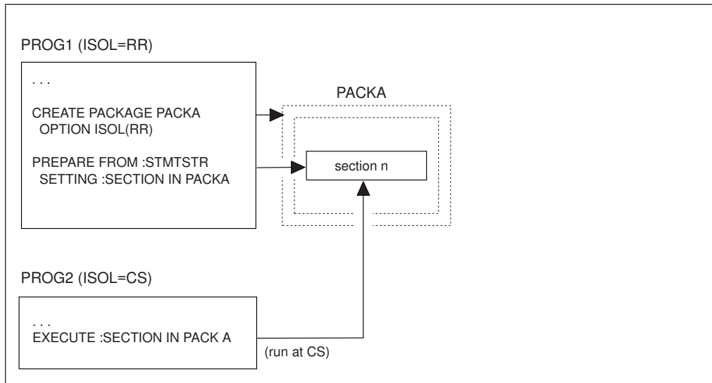
Figure 132. Dropping and Re-creating PACKA Without Reprocessing PROG2
