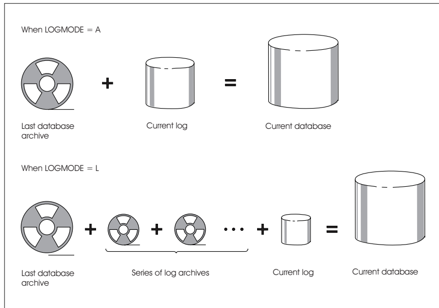
Figure 69. Relationships among the Archives, the Log, and the Database
