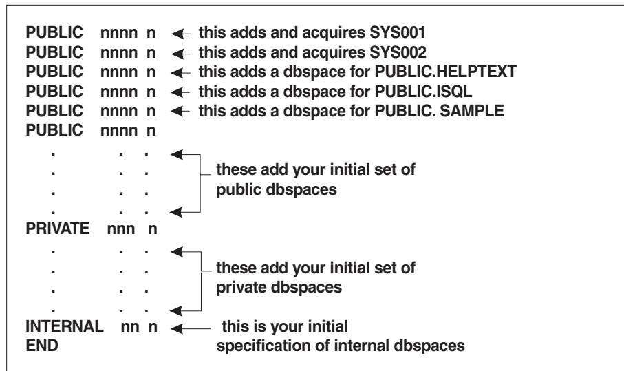
Figure 91. Input Records for Initial Dspace Definitions
