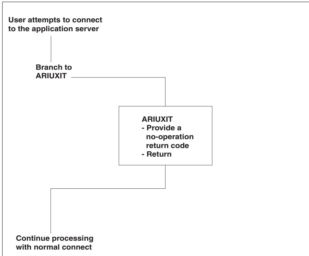
Figure 105. The Database Manager Branching to ARIUXIT
