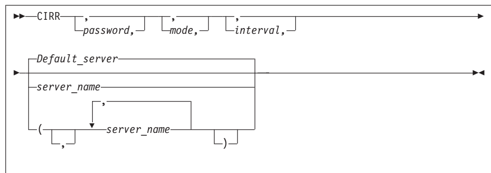
Figure 42. CIRR Transaction Syntax
