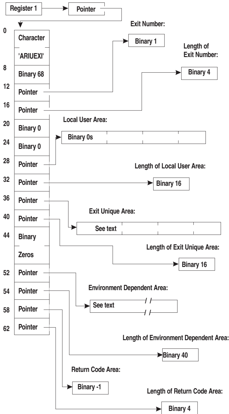
Figure 106. Summary of ARIUEXI Parameter List and Associated Areas
