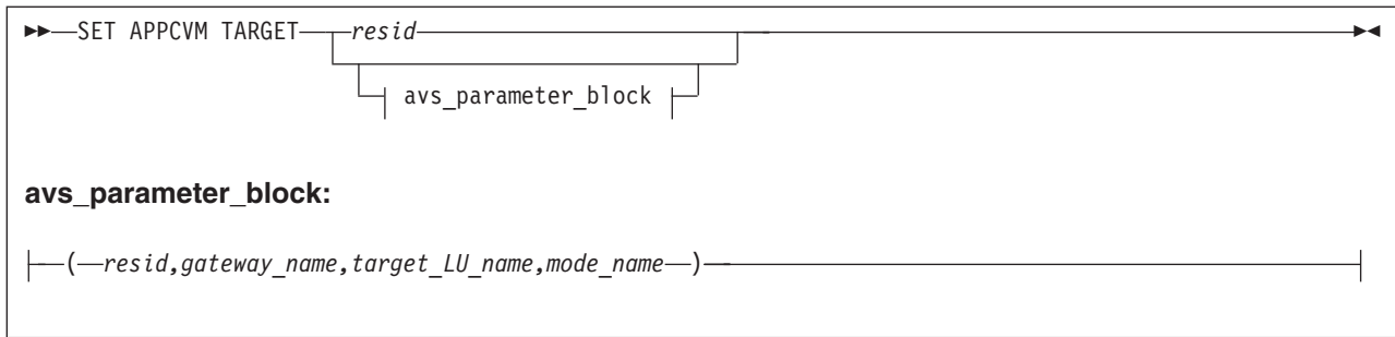
Figure 28. SET APPCVM Command
