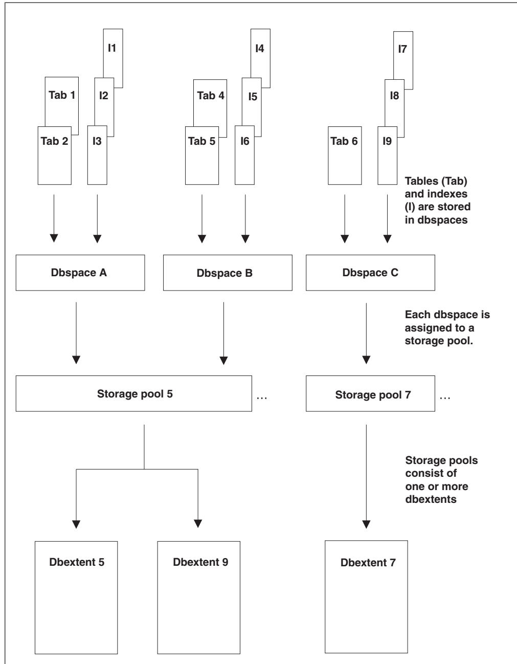
Figure 57. Physical Database Concepts
