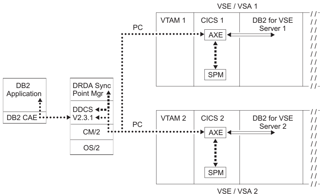
Figure 123. DB2 Server for VSE Distributed Unit of Work
