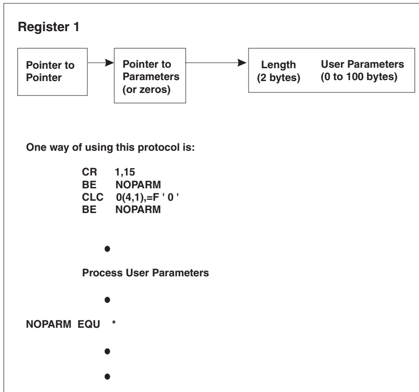
Figure 24. Passing User Parameters to a User Application Program
