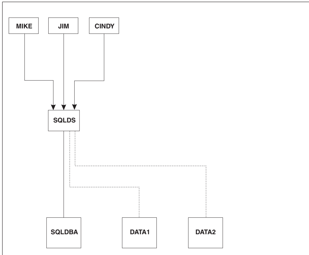
Figure 85. One Database Partition Accessing One Database
