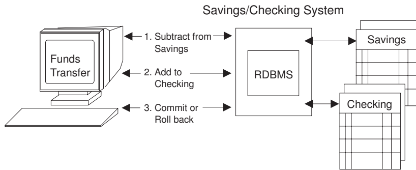
Figure 117. Remote unit of work
