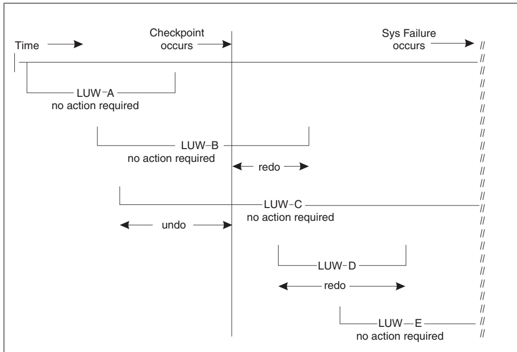
Figure 68. LUW Recovery Actions
