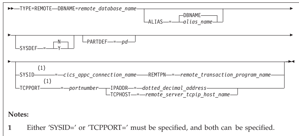
Figure 10. REMOTE Type Entry
