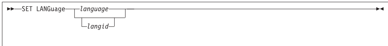
Figure 104. The SET LANGUAGE Command
