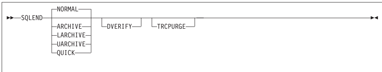
Figure 27. SQLEND Operator Command
