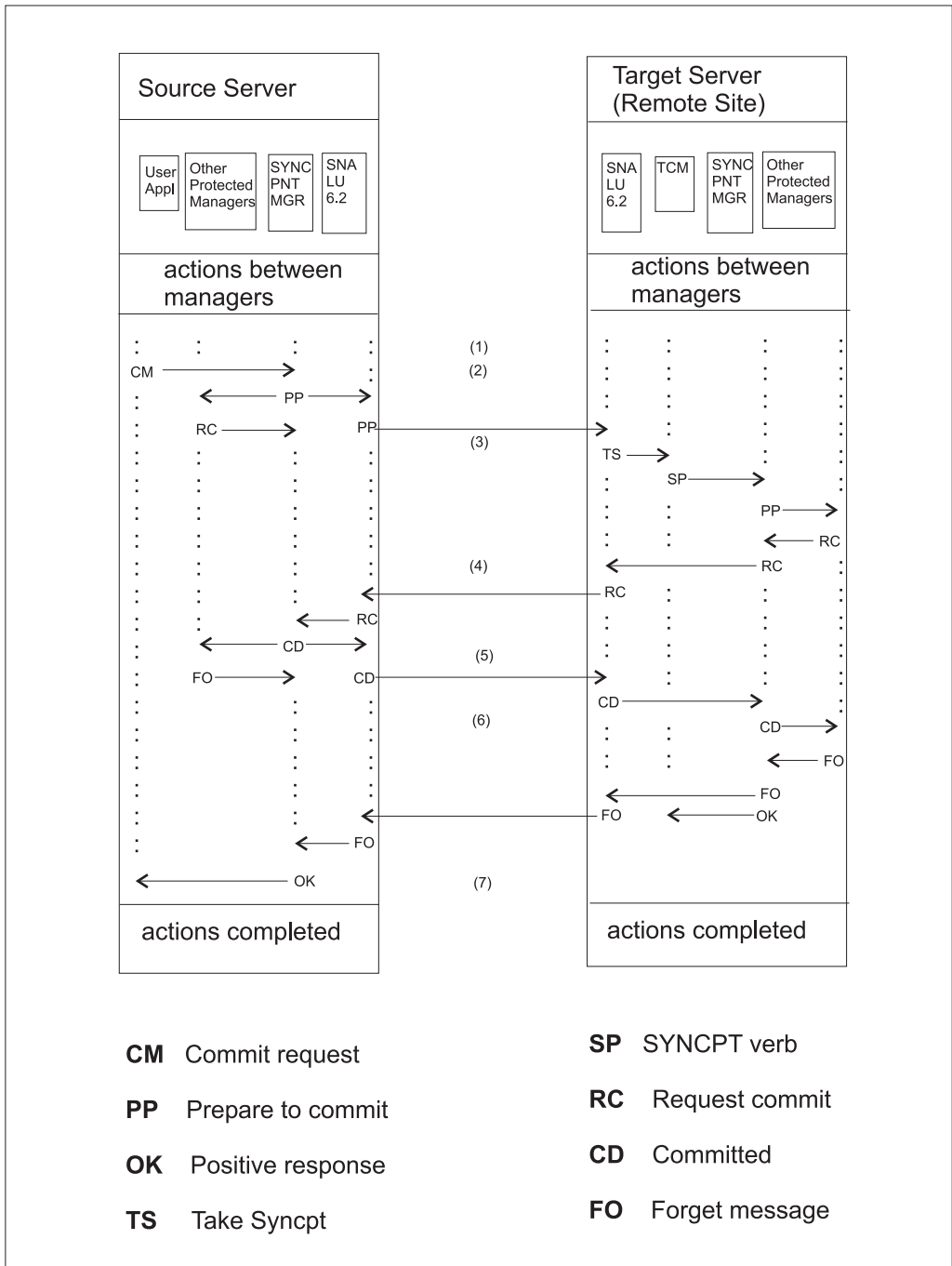
Figure 122. Successful Two-Phase Commit
