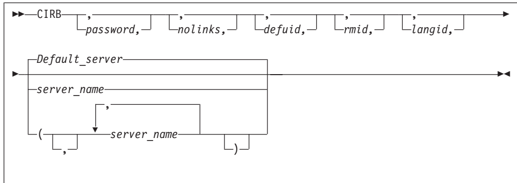
Figure 29. CIRB Transaction Syntax
