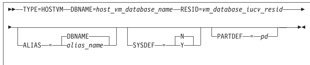
Figure 9. HOSTVM Type Entry
