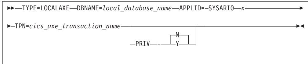
Figure 11. LOCALAXE Type Entry
