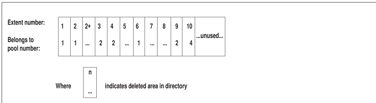
Figure 66. Dbextent Control Area in the Database Directory
