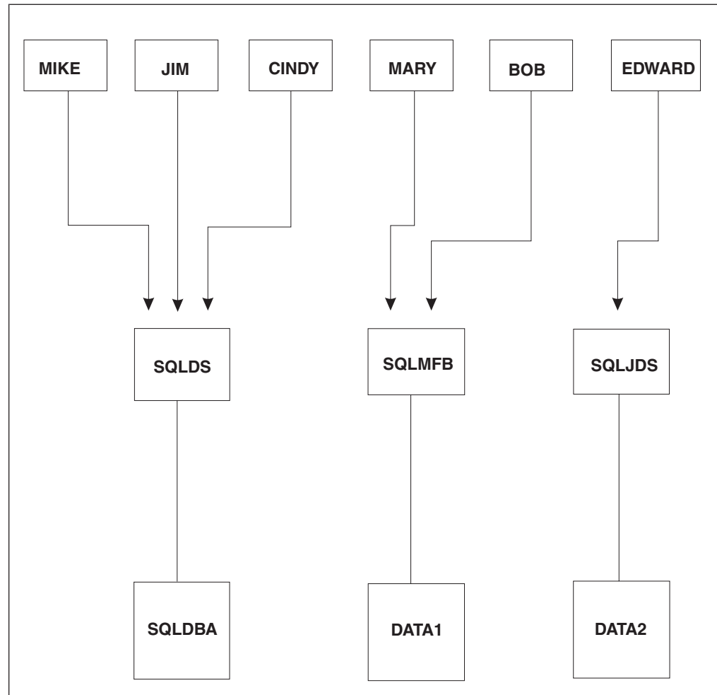
Figure 86. Multiple Users Accessing Multiple Databases
