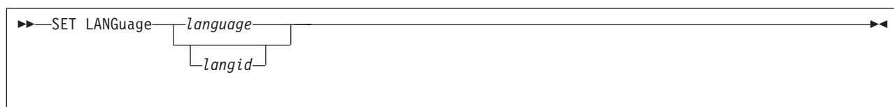
Figure 108. The SET LANGUAGE Command
