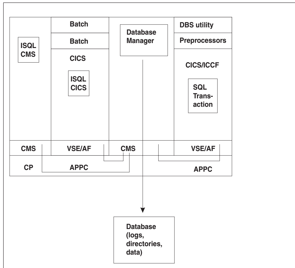
Figure 97. VSE Guest Sharing on One Processor
