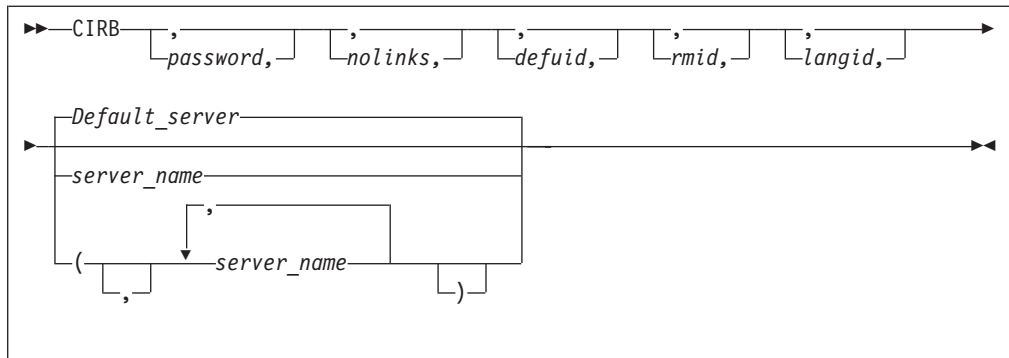
Figure 20. CIRR Transaction Syntax
