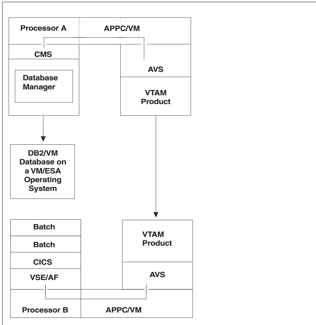
Figure 99. VSE Guest Sharing with VTAM Product and AVS
