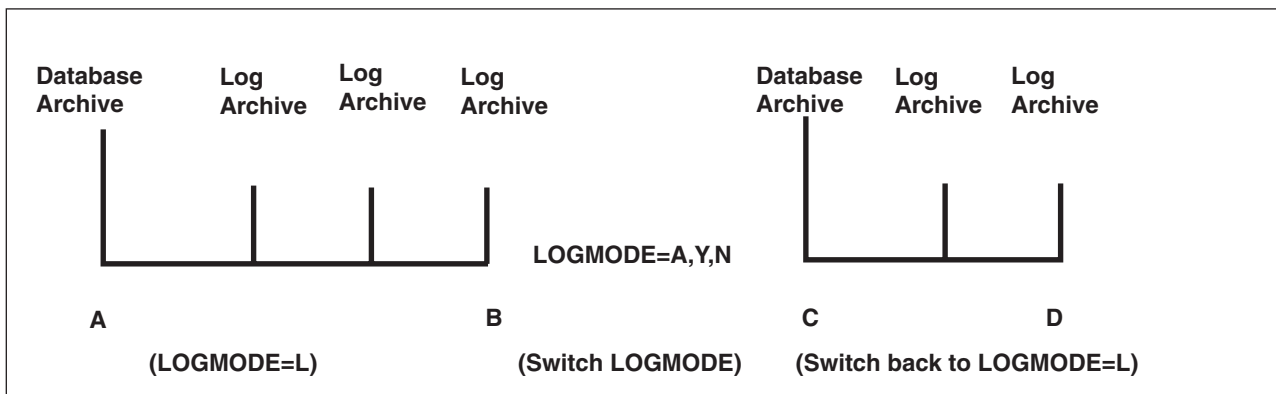
Figure 75. Log Archive Continuity
