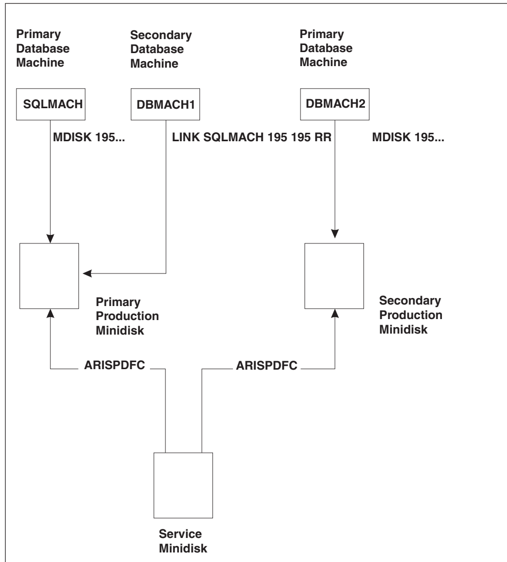
Figure 83. Types of Database Machines
