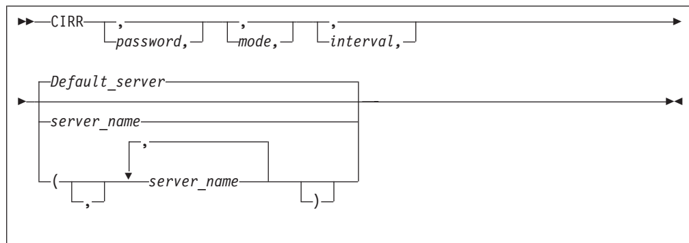
Figure 33. CIRR Transaction Syntax
