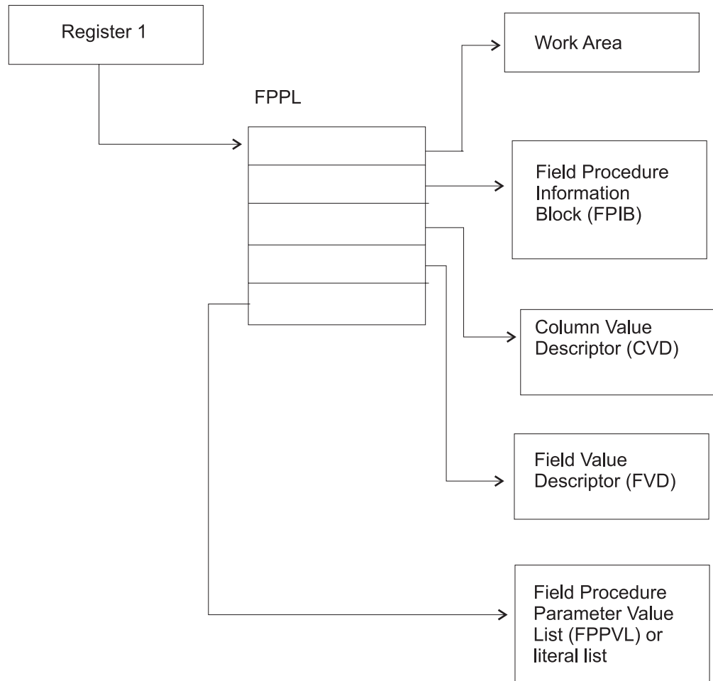
Figure 117. Field Procedure Parameter List
