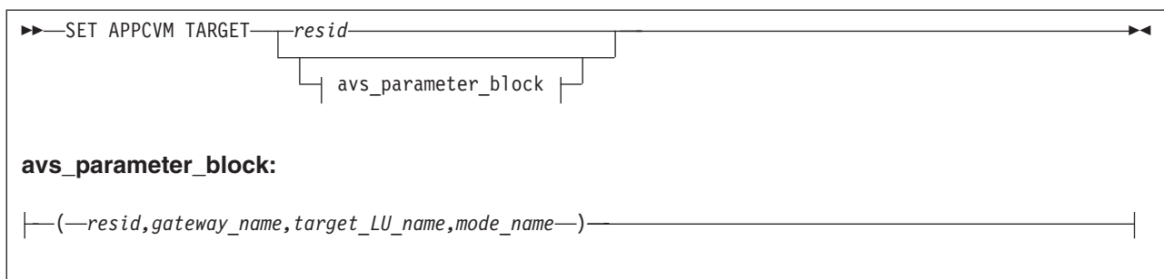
Figure 19. SET APPCVM Command
