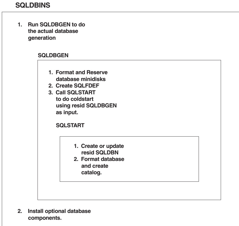
Figure 96. Summary of Database Generation Process
