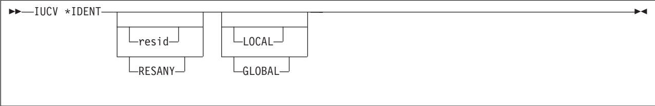
Figure 4. IUCV *IDENT Syntax
