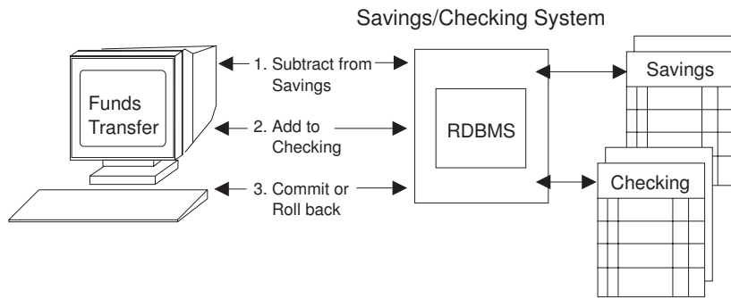
Figure 119. Remote unit of work
