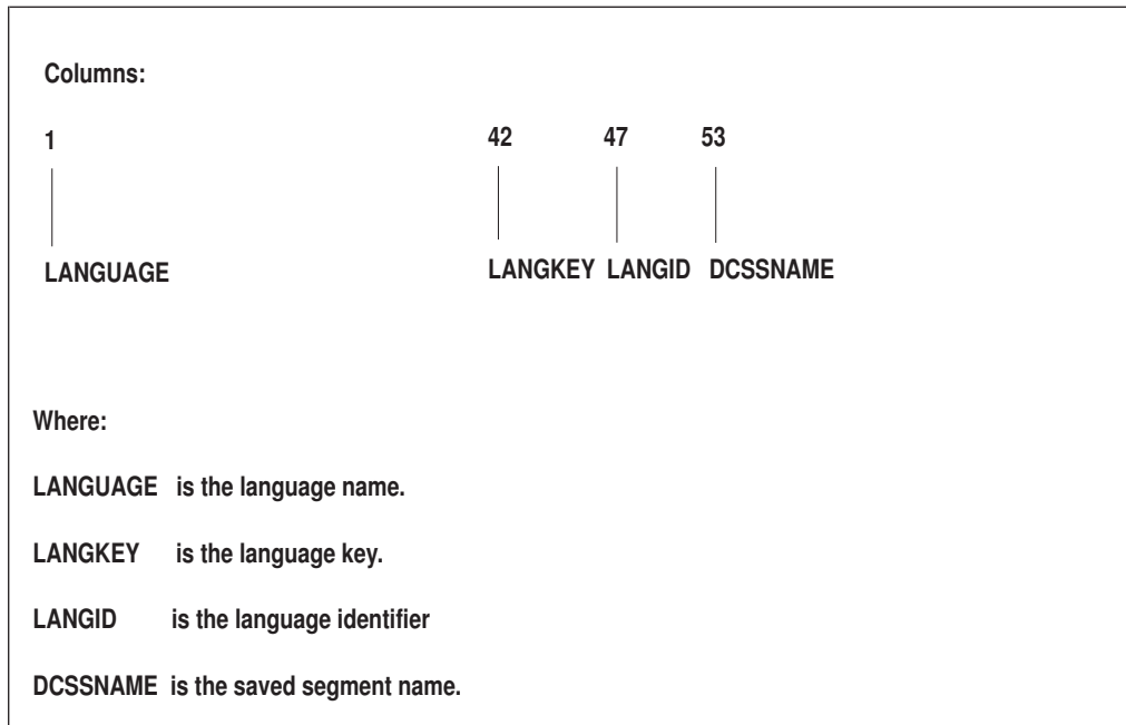
Figure 71. The ARISNLSC MACRO
