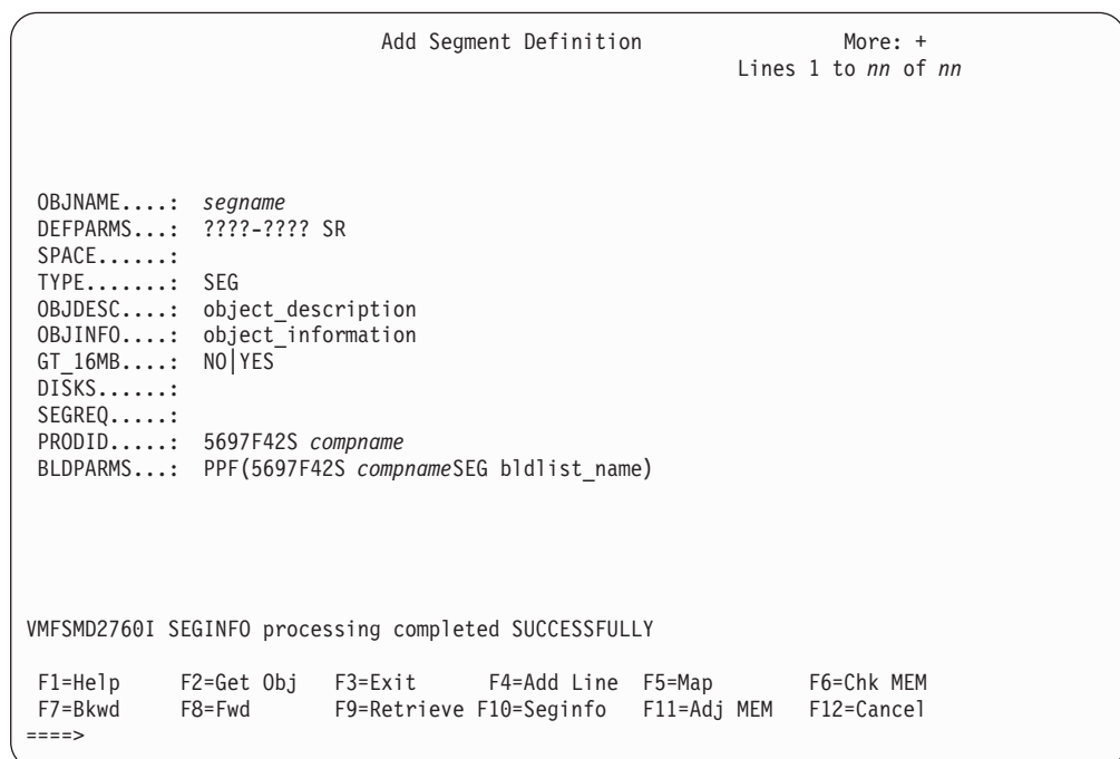
Figure 66. Add Segment Definition Panel Showing the New Segment Information
