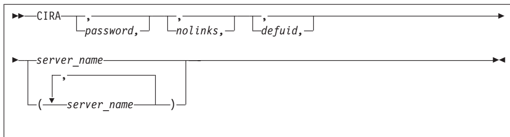
Figure 25. CIRA Transaction Syntax
