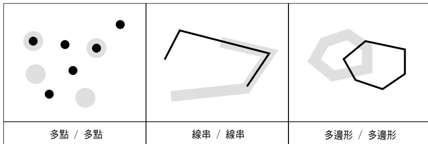
圖 17. ST_Overlaps
