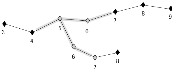
圖 26. LocateBetween
