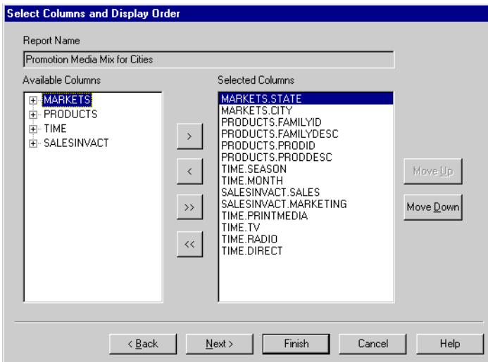
Abbildung 189. Dialogfenster "Select Columns and Display Order"
