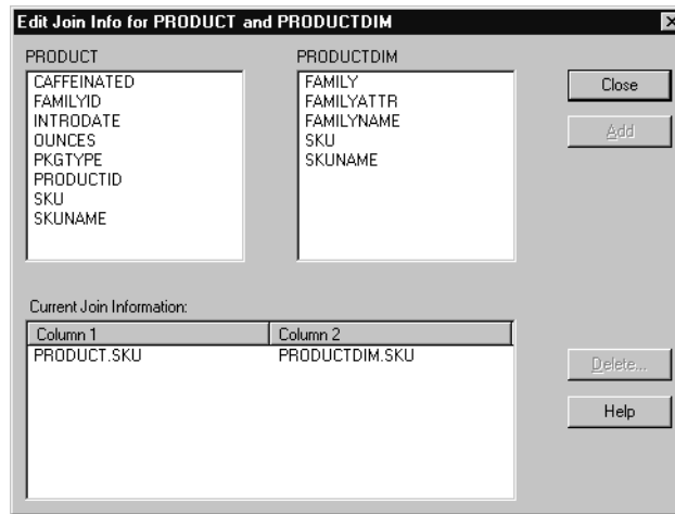
Figure 9-6: Specifying or Verifying Join Information for a New Join Between Dimension Tables
