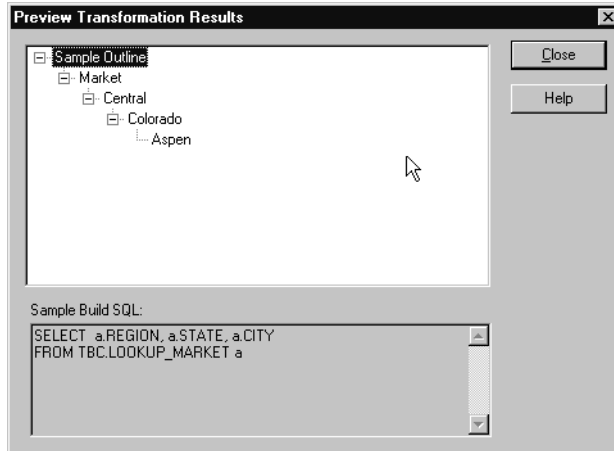
Figure 10-19: Viewing a Sample Hyperion Essbase Outline
