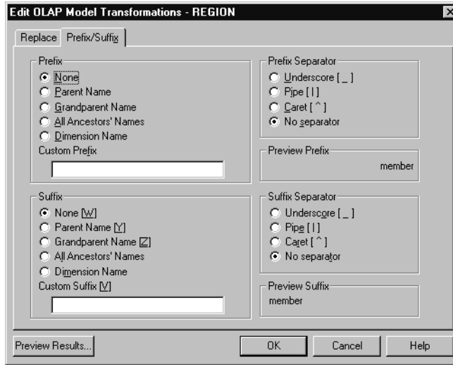
Figure 10-18: Prefix/Suffix Tab
