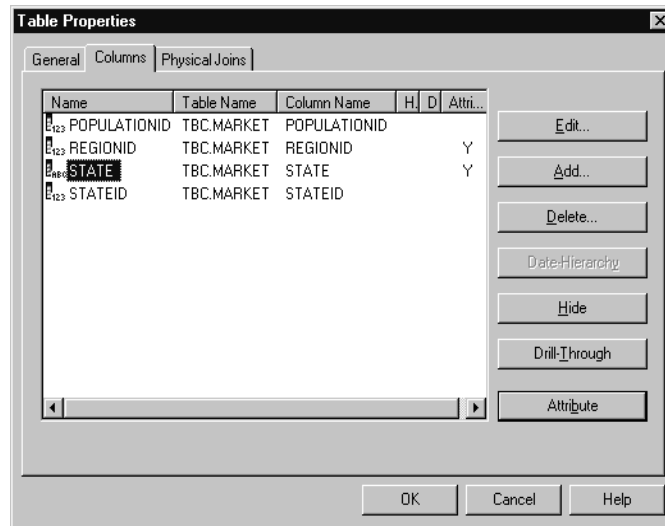
Figure 8-4: Attribute-Enabled Column
