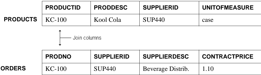
Figure 9-2: Join Columns Between Two Tables
