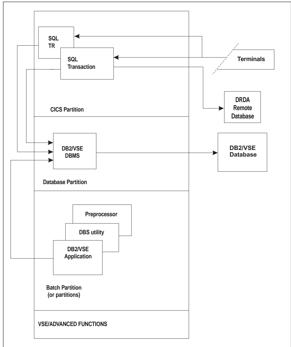
Figure 2. Online Transaction Processing Configuration
