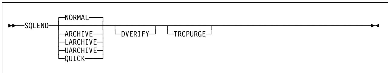
Figure 23. SQLEND Operator Command
