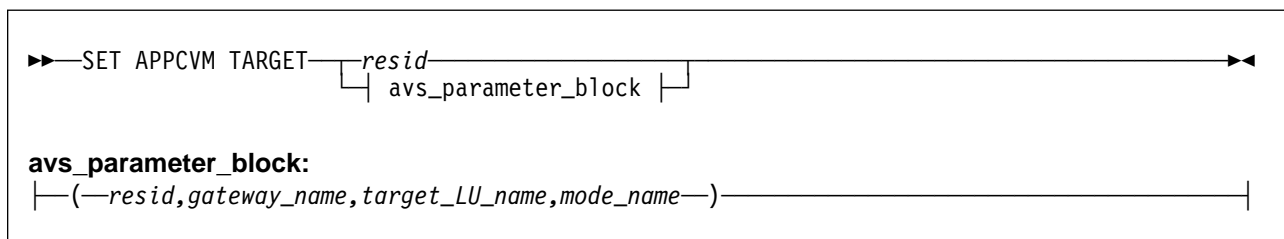
Figure 24. SET APPCVM Command
