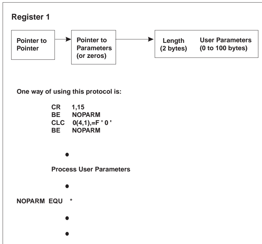
Figure 20. Passing User Parameters to a User Application Program
