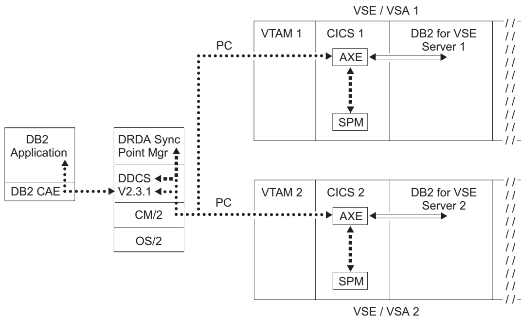
Figure 118. DB2 Server for VSE Distributed Unit of Work
