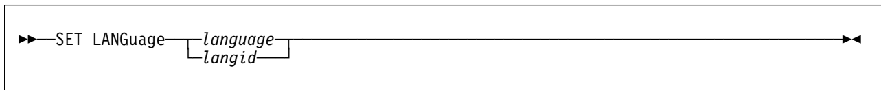
Figure 100. The SET LANGUAGE Command
