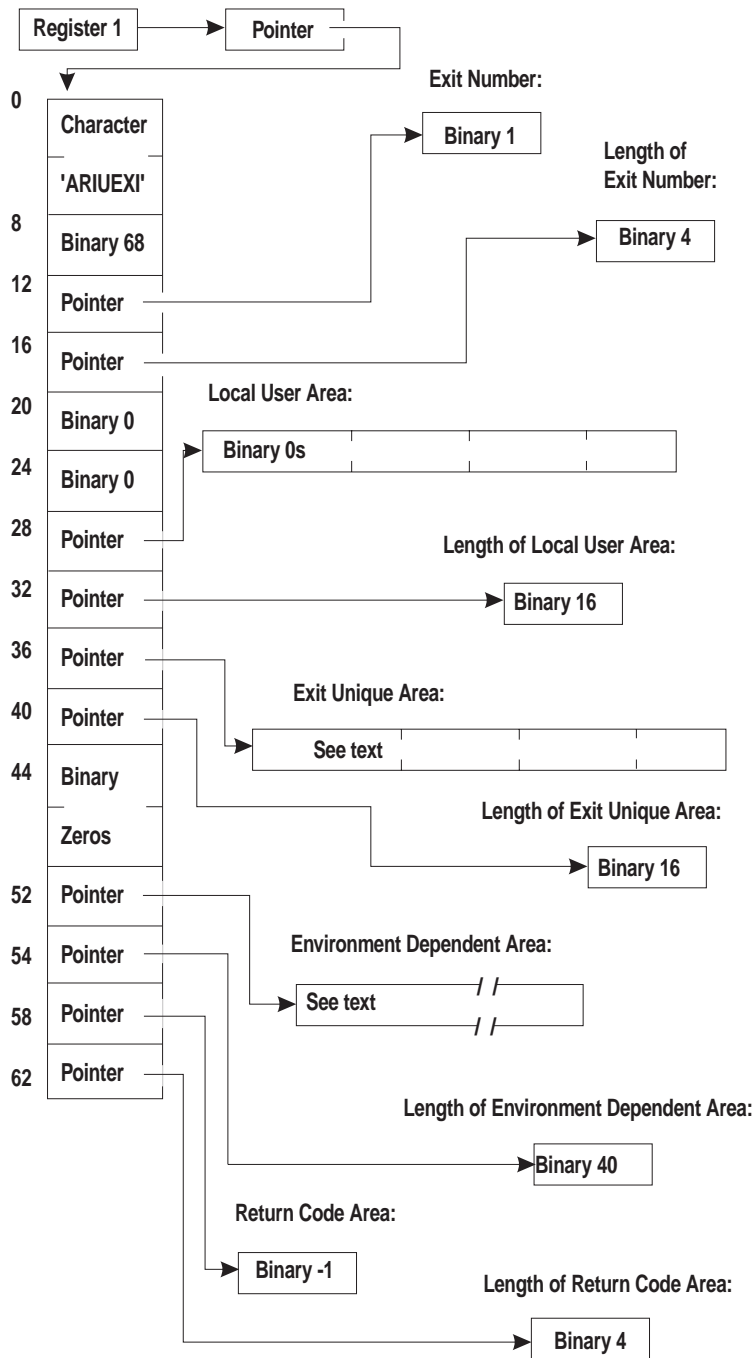
Figure 102. Summary of ARIUEXI Parameter List and Associated Areas
