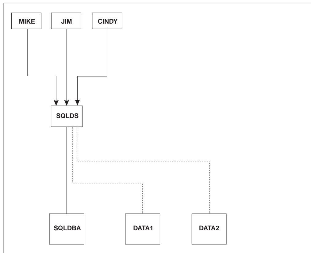
Figure 81. One Database Partition Accessing One Database
