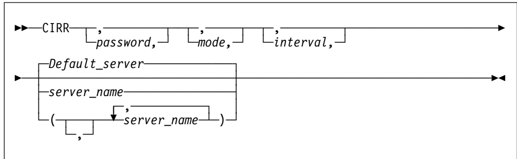
Figure 38. CIRR Transaction Syntax
