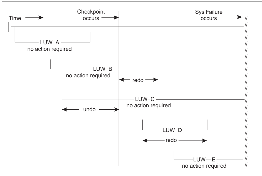
Figure 64. LUW Recovery Actions
