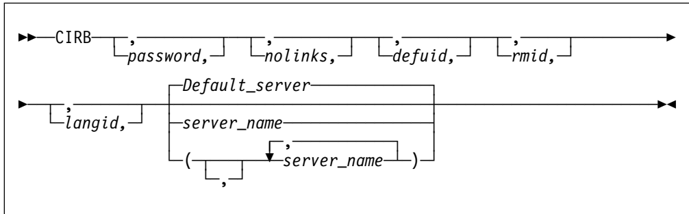
Figure 25. CIRB Transaction Syntax
