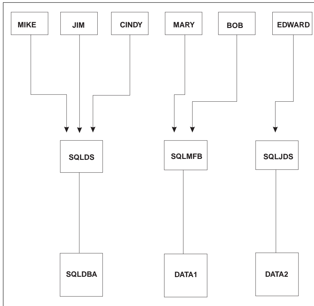
Figure 82. Multiple Users Accessing Multiple Databases
