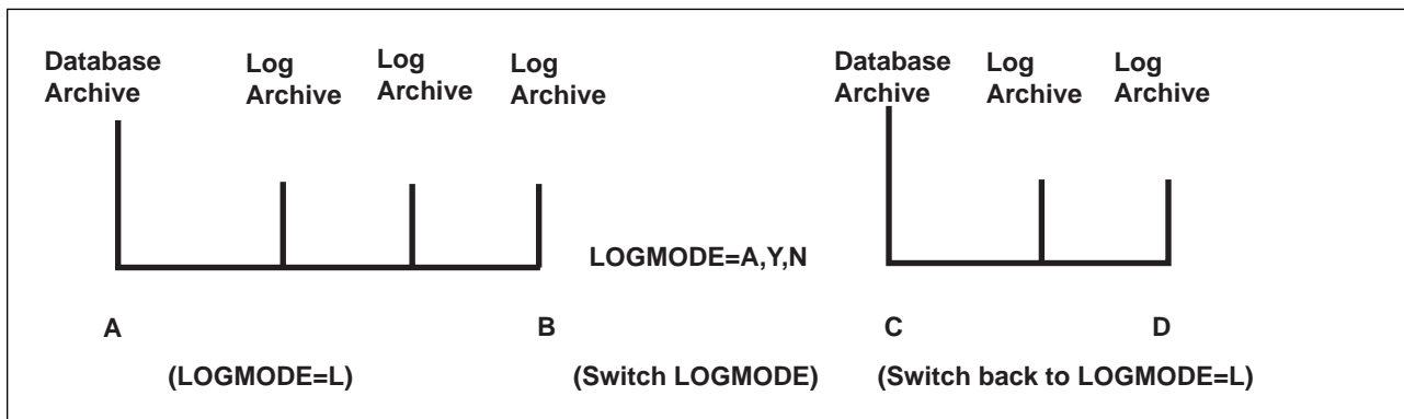
Figure 69. Log Archive Continuity
