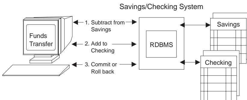
Figure 115. Remote unit of work
