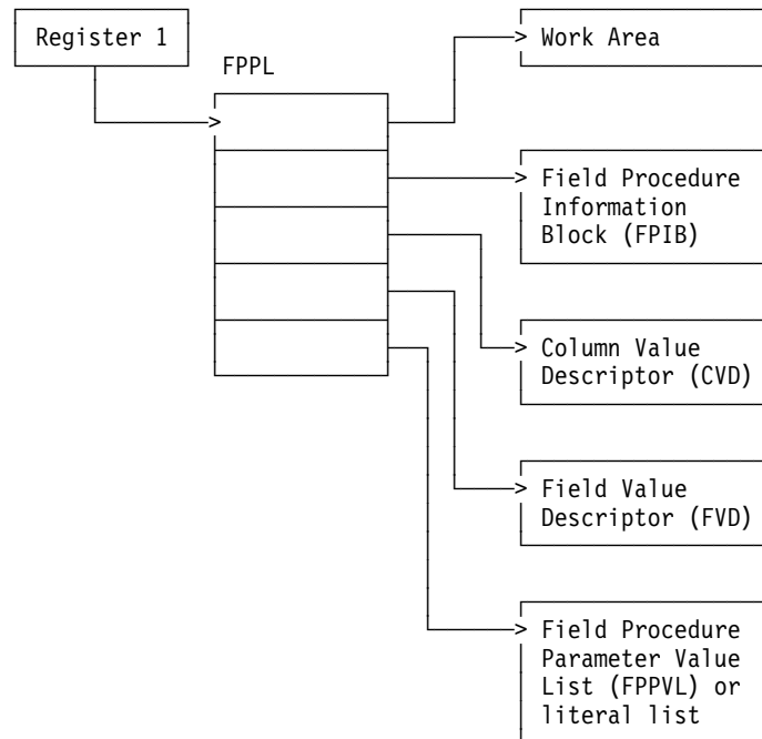
Figure 111. Field Procedure Parameter List
