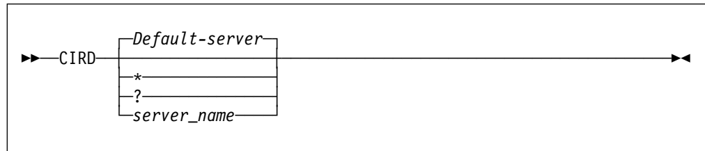
Figure 41. CIRD Transaction Syntax
