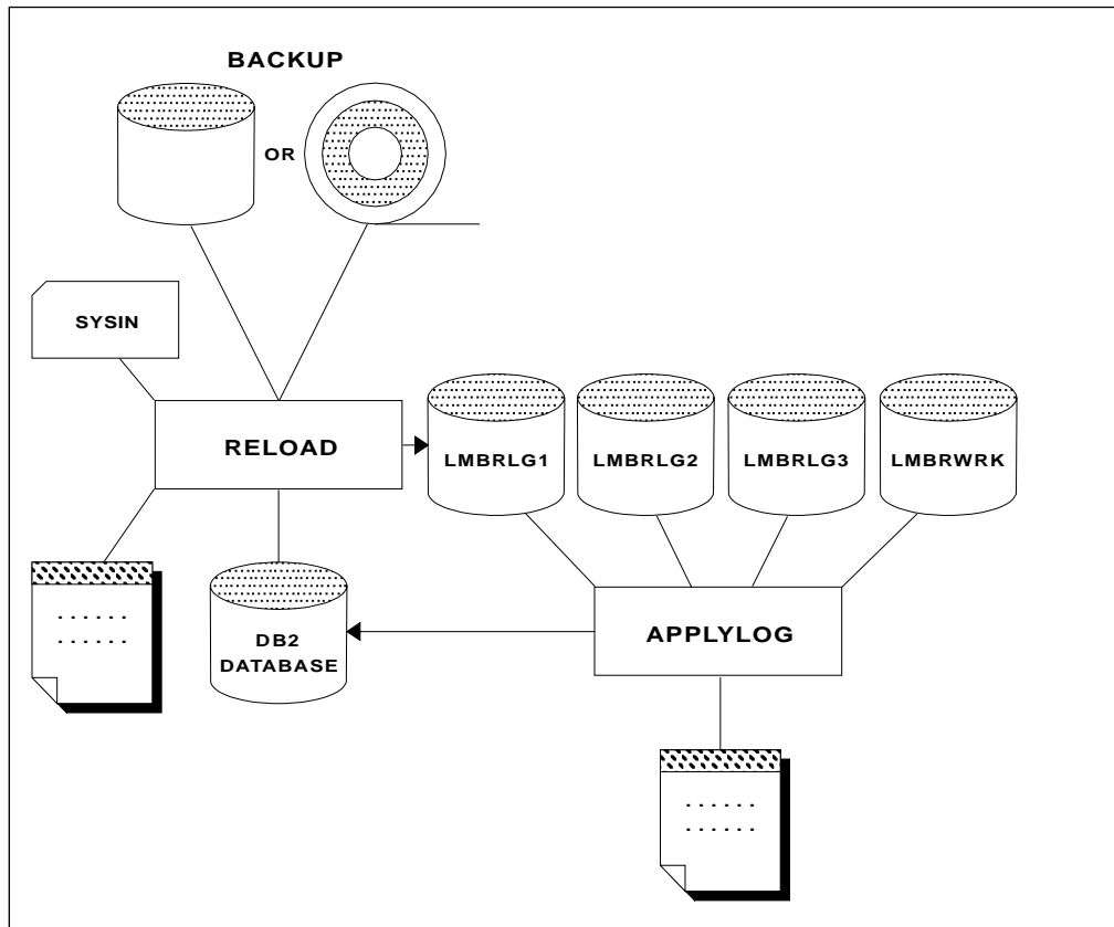
Figure 130. Apply Changes From the Log To the Reloaded Tables
