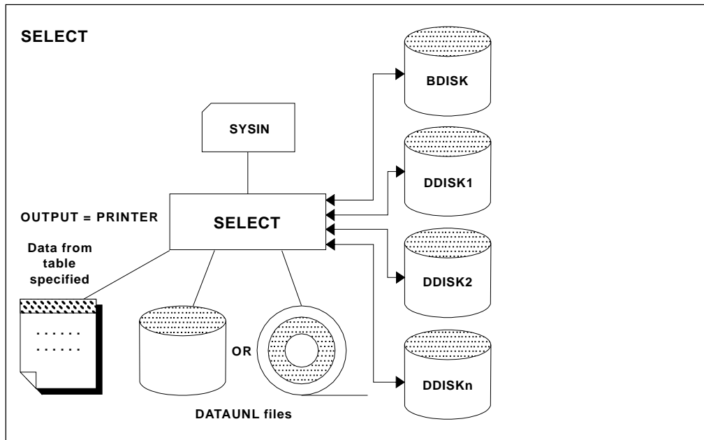
Figure 135. Overview of the SELECT function
