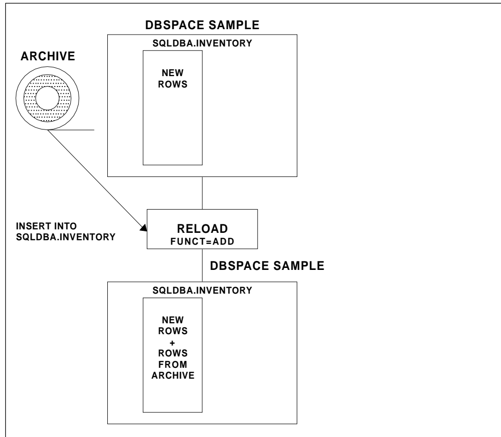
Figure 115. RELOADing a Table with the ADD Parameter
