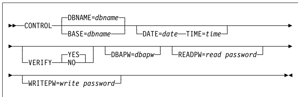
Figure 165. CONTROL statement
