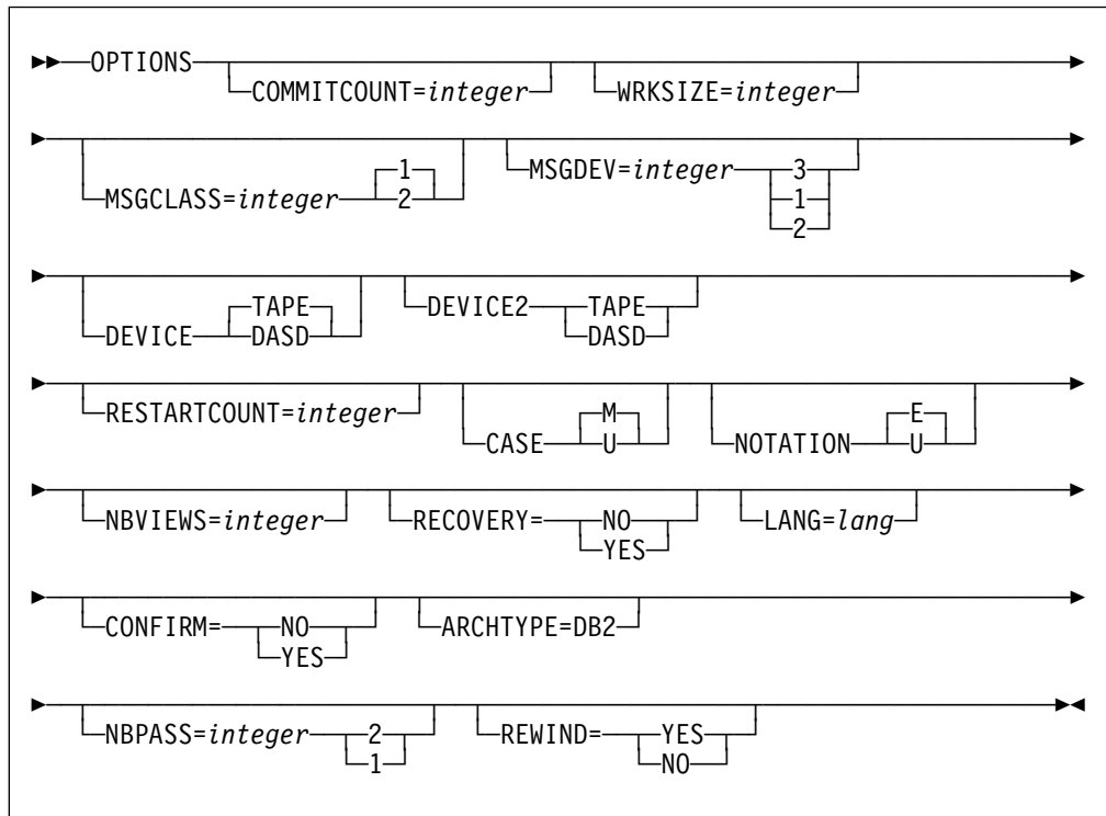
Figure 164. OPTIONS statement
