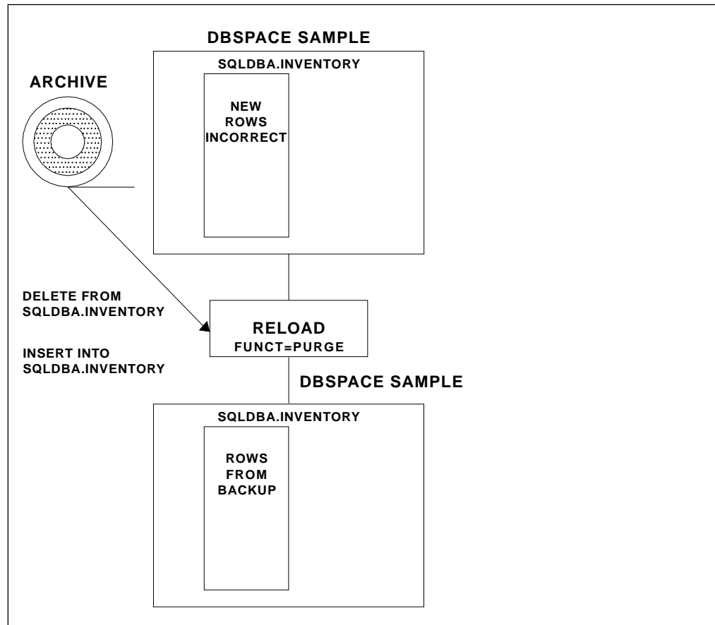
Figure 113. RELOADing a Table with the PURGE Parameter
