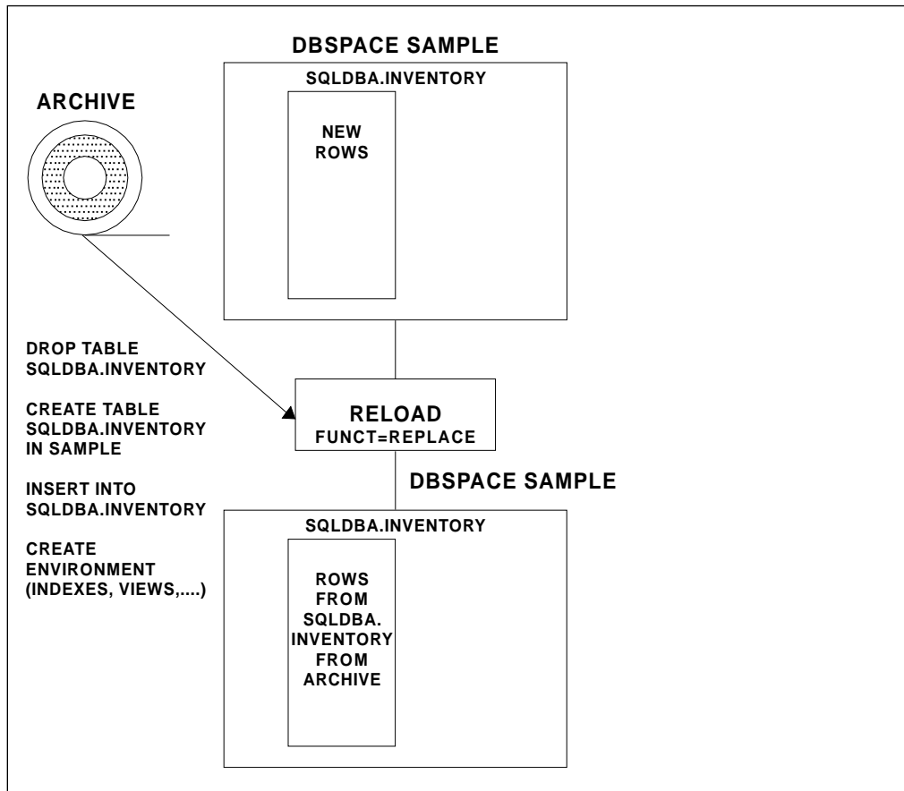
Figure 116. RELOADing a Table with the REPLACE Parameter
