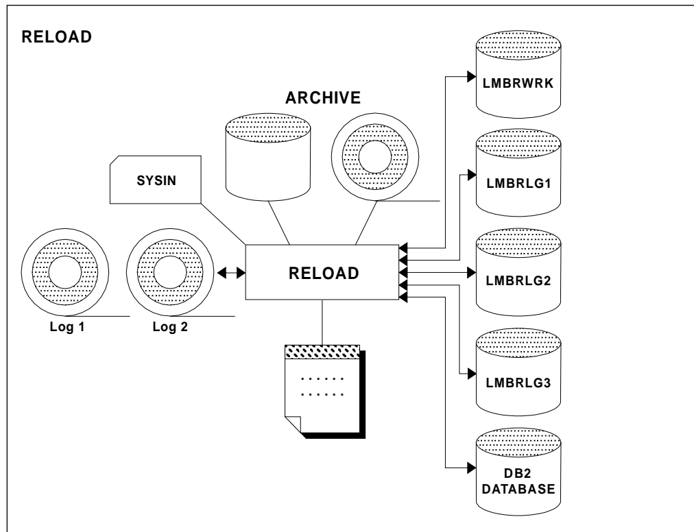
Figure 118. Possible Input Sources for RELOADing Tables with Forward Recovery
