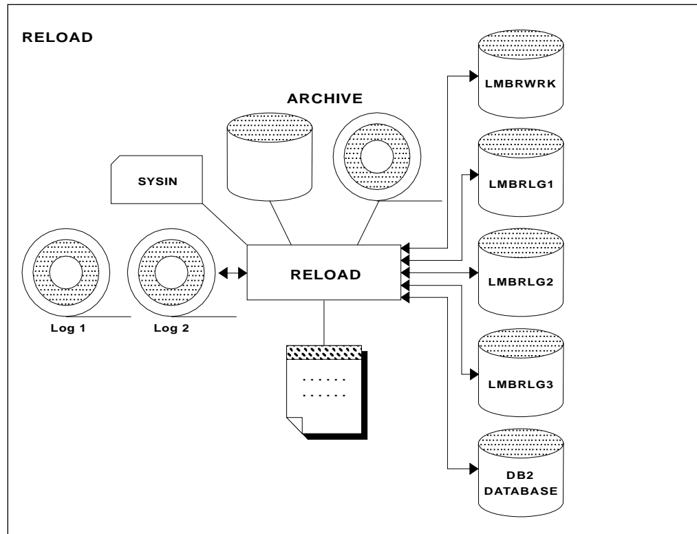
Figure 244. Possible Input Sources for RELOADing Tables with Forward Recovery
