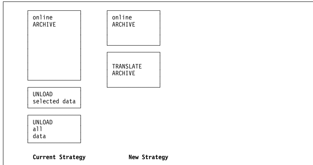
Figure 2. Migration from Online DB2 Archive
