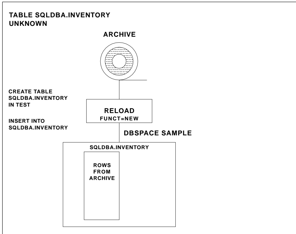
Figure 114. RELOADing a Table with the NEW Parameter
