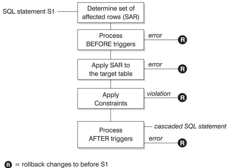
Figure 18. Processing an SQL statement with associated triggers and constraints
