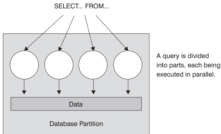
Figure 3. Intra-Partition Parallelism
