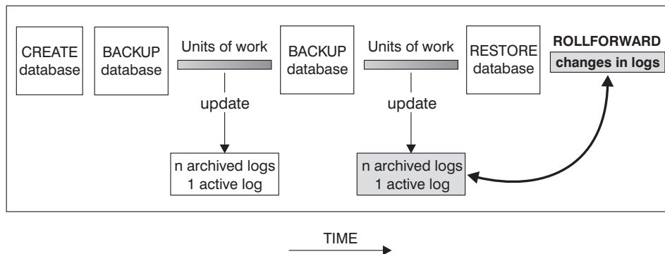
Figure 34. Roll-Forward Recovery
