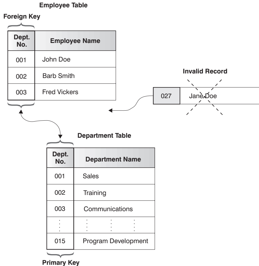
Figure 4. Foreign and Primary Constraints Define Relationships and Protect Data
