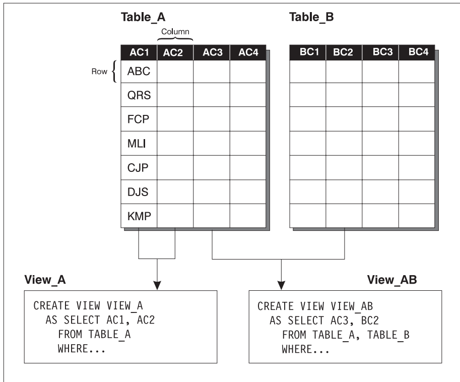
Figure 2. Relationship Between Tables and Views
