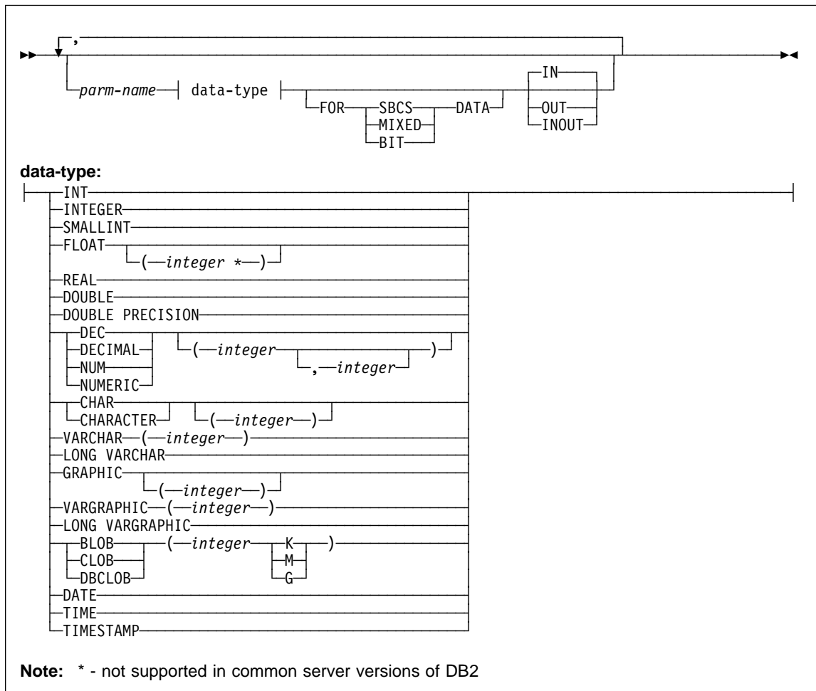
Figure 19. PARMLIST String Syntax. This PARMLIST syntax diagram combines the data types supported for both DB2 for MVS/ESA and for common server versions of DB2.
