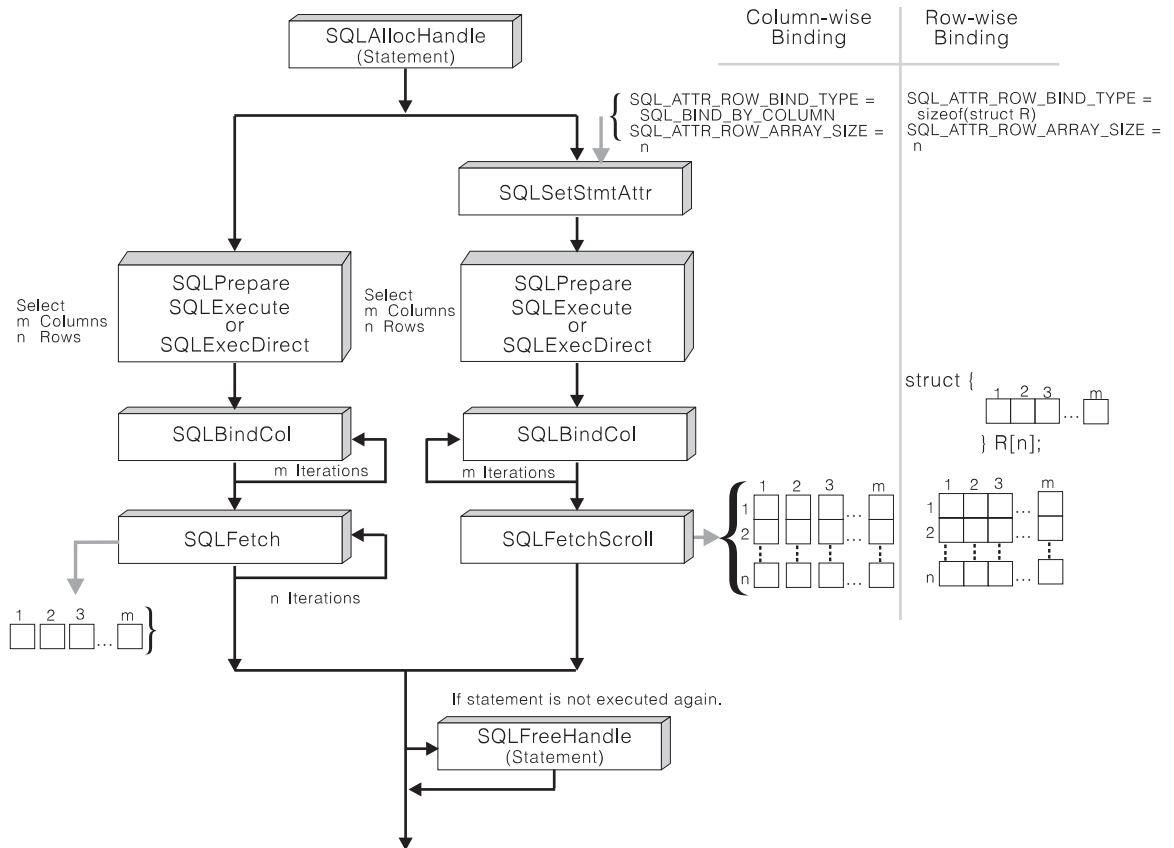
Figure 14. Array Retrieval
