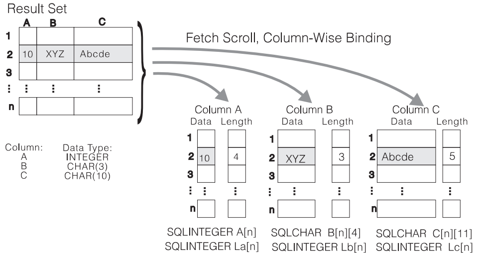
Figure 12. Column-Wise Binding
