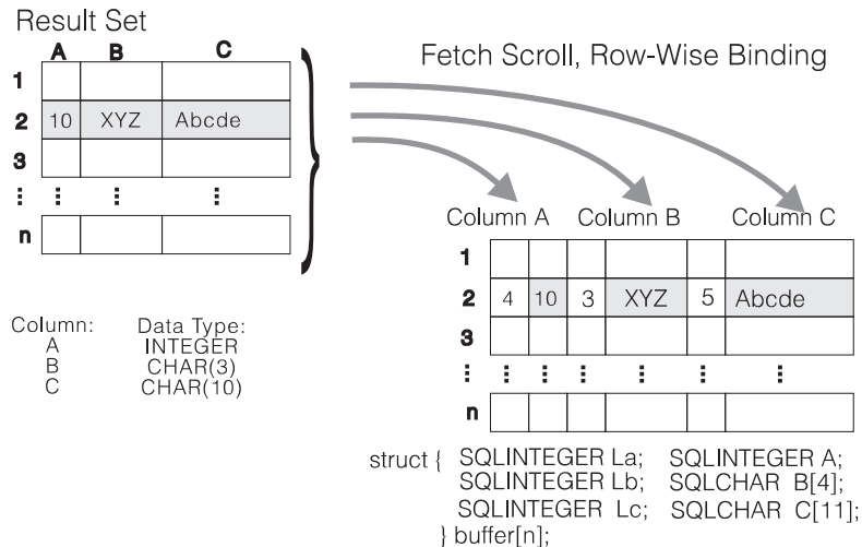
Figure 13. Row-Wise Binding
