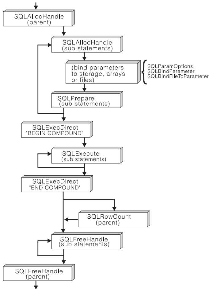
Figure 15. Compound SQL
