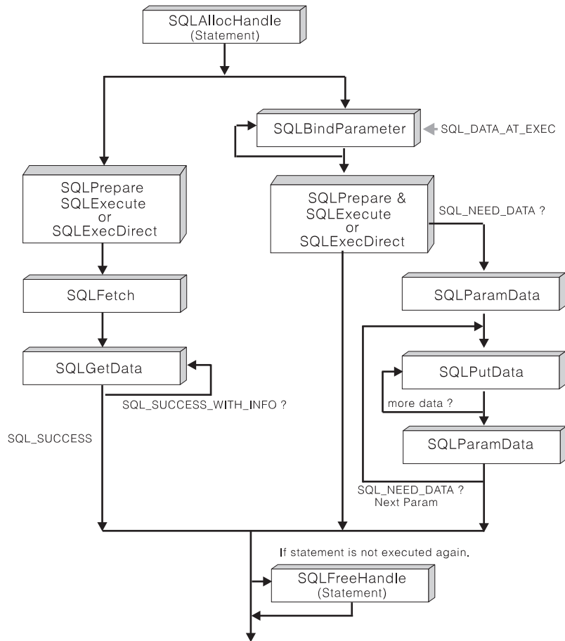
Figure 9. Piecewise Input and Retrieval
