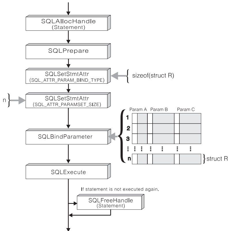
Figure 11. Row-Wise Array Insert
