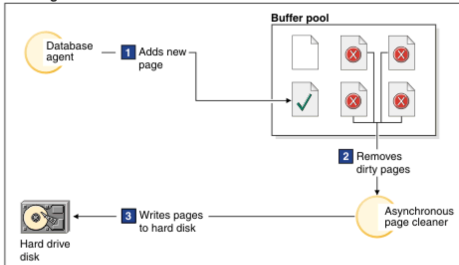
Figure 19. Asynchronous page cleaning
