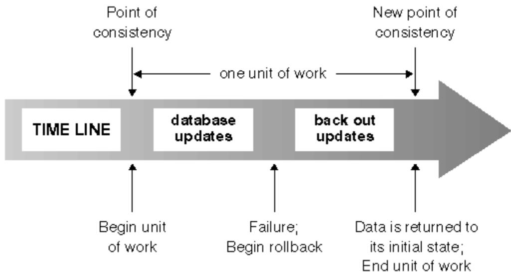
Figure 22. Unit of work with a ROLLBACK statement
