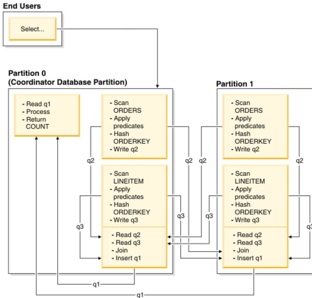
Figure 30. Directed Inner-Table and Outer-Table Join Example
