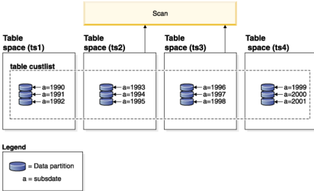
Figure 33. The performance benefits of data partition elimination
