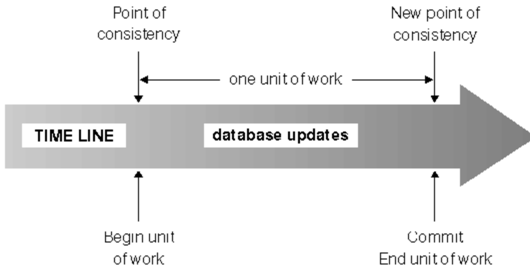
Figure 21. Unit of work with a COMMIT statement
