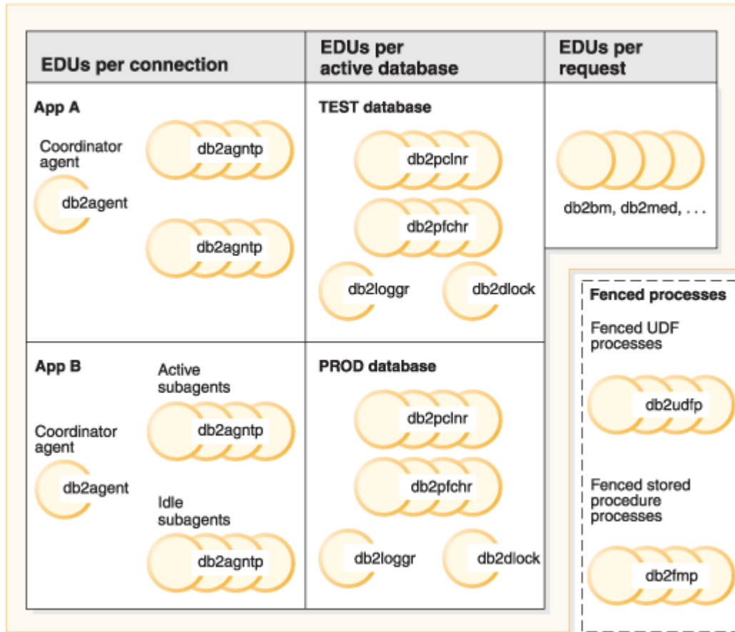
Figure 6. EDUs in the database server
