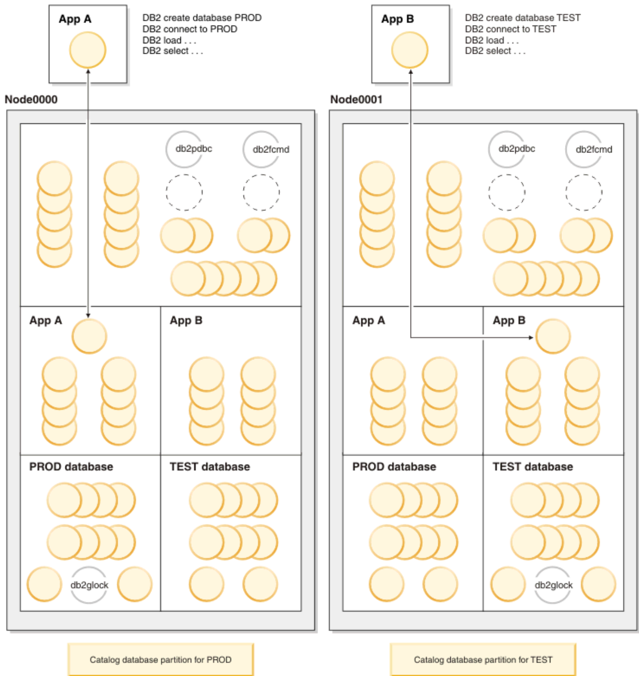
Figure 7. Process model for multiple database partitions
