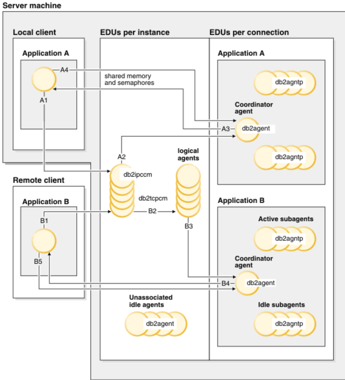
Figure 5. Client-server processing model overview
