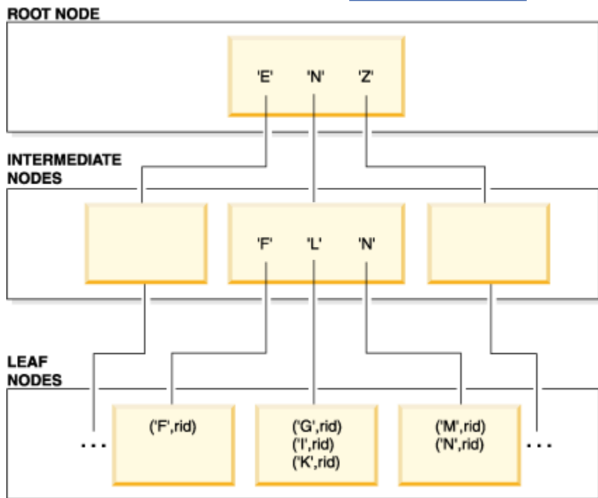
Figure 11. Structure of a B+ Tree Index
