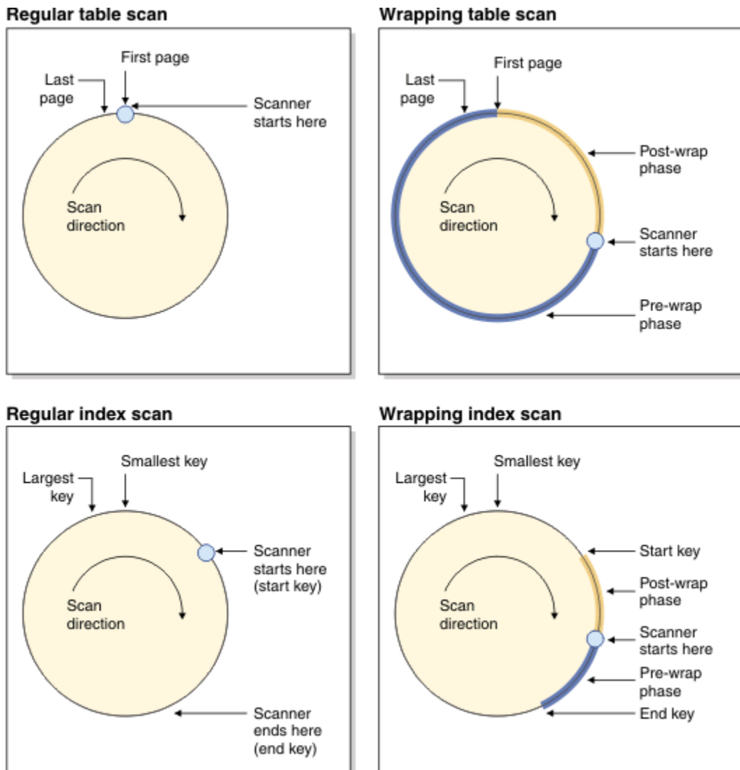
Figure 25. Conceptual view of regular and wrapping scans
