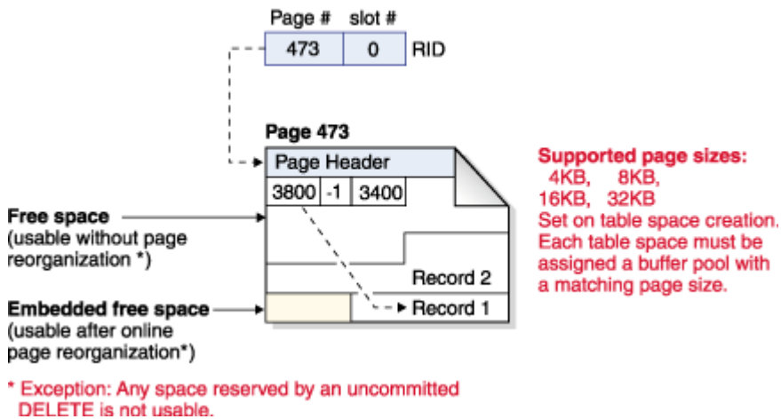
Figure 9. Data page and record ID (RID) format
