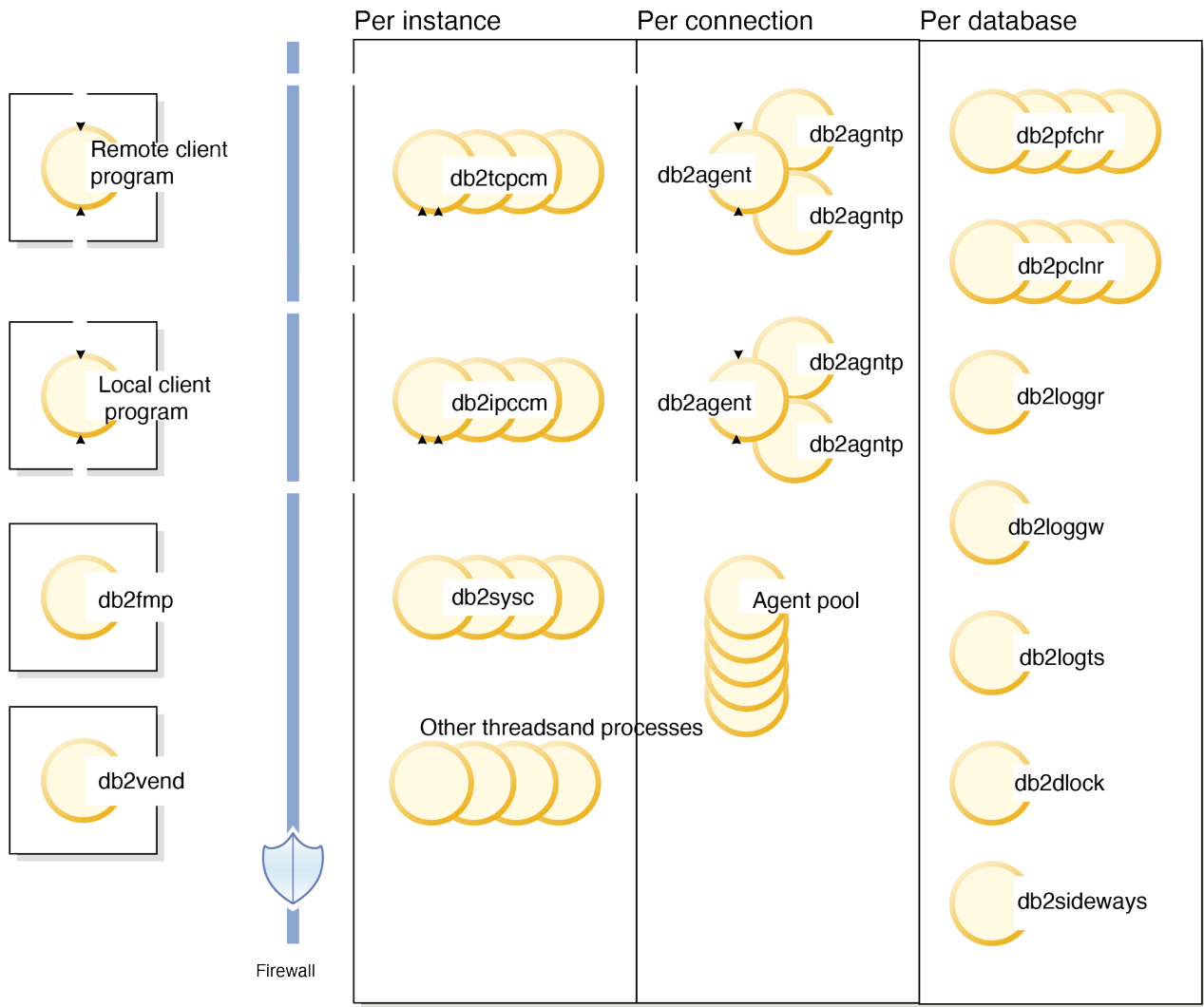
Figure 4. Process model for Db2 database systems
