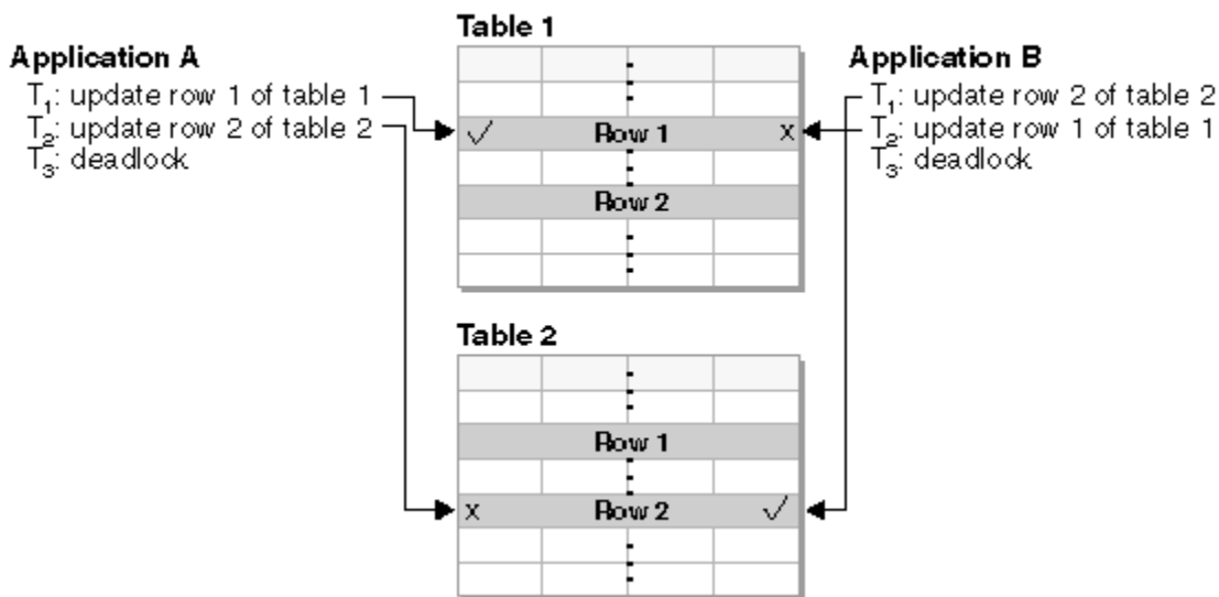
Figure 23. Deadlock between applications
