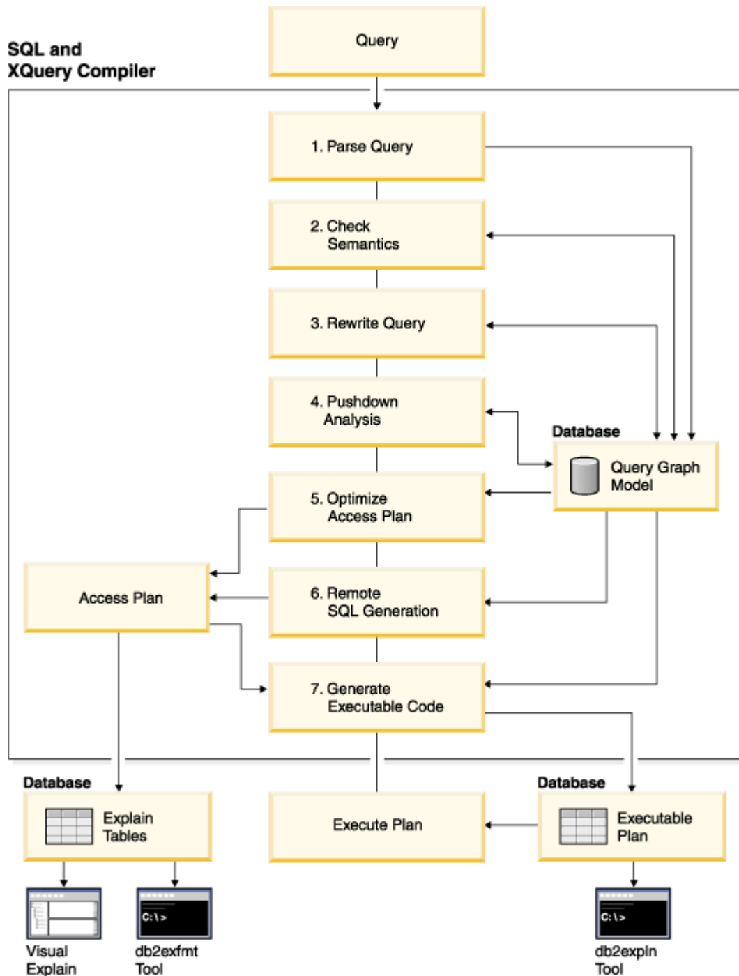
Figure 24. Steps performed by the SQL and XQuery compiler
