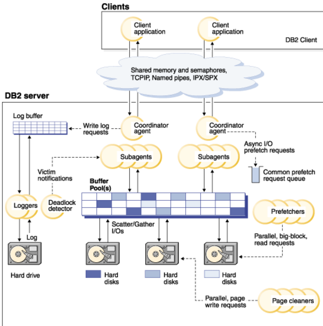
Figure 3. Client connections and database server components
