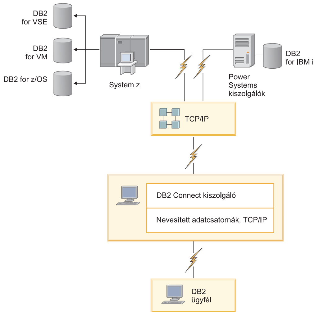
2. ábra: DB2 Connect Enterprise Edition
